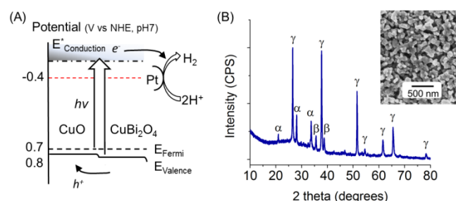
Figure 1. (A) Schematic energy diagram of the estimated band-edge positions of CuO|CuBi 2 O 4 |Pt heterojunction. (B) Powder X-ray diffraction patterns of CuO|CuBi 2 O 4 heterojunction (α=CuBi 2 O 4 , PDF#48-1886; β=CuO, PDF#44-0706; and γ=FTO). Inset in (B) shows an SEM image of CuO|CuBi 2 O 4 electrode surface.
