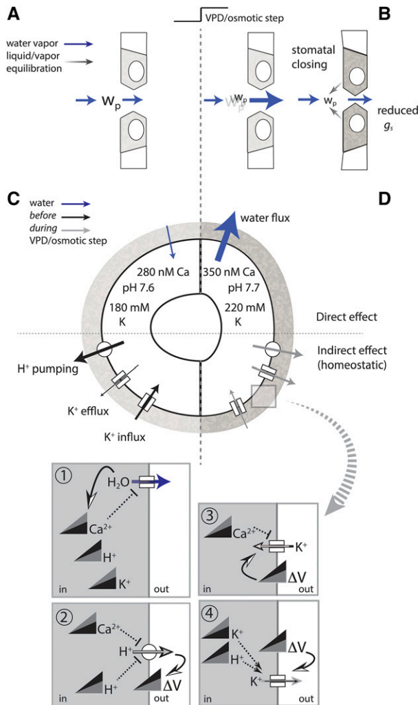
Figure 8. A Step Decrease in Partial Vapor Pressure of Water at p , w_p , or a Step Increase in the Osmotic Solute Load of the Apoplast Drives Stomatal Closure via Water Flux from the Guard Cell and Homeostatic Adjustment in Guard Cell Transport.
