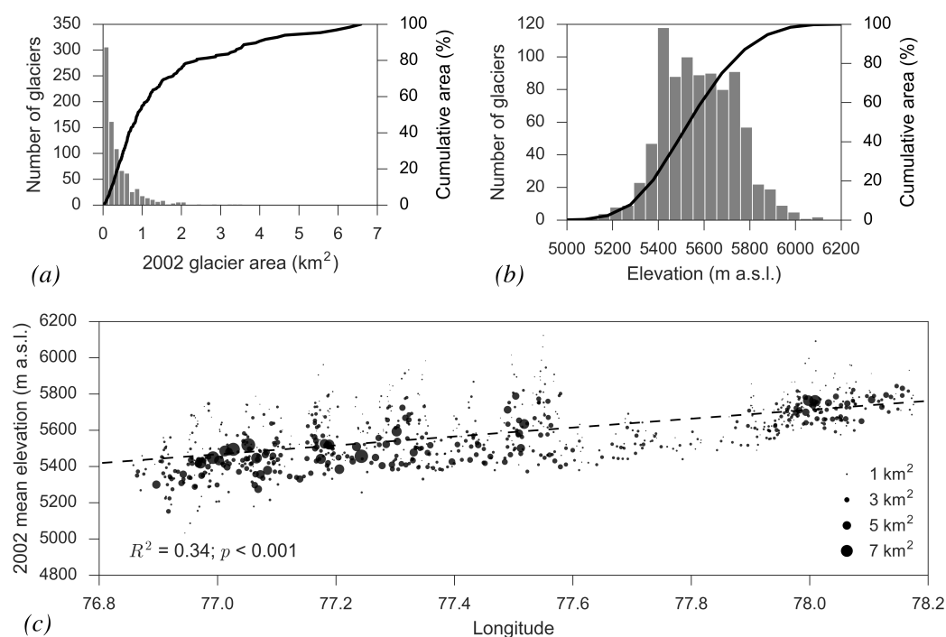
Figure 2. Graphs of glacier characteristics: (a) Histogram and cumulative glacier area line for 2002 glacier area; (b) Histogram and cumulative glacier area line for 2002 glacier mean elevation; (c) change in glacier mean elevation with longitude, with points sized according to glacier area.
