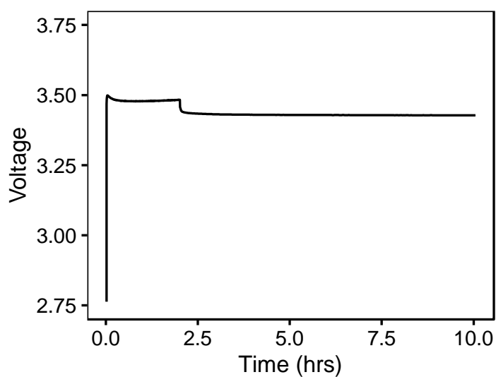
Figure S20. An example of the electrochemistry for the OCV experiments – Galvanostatic plating for 2 hours followed with a rest period at the OCV for an in situ NMR experiment in LP30 + FEC with 0.5 mA/cm 2 current density
