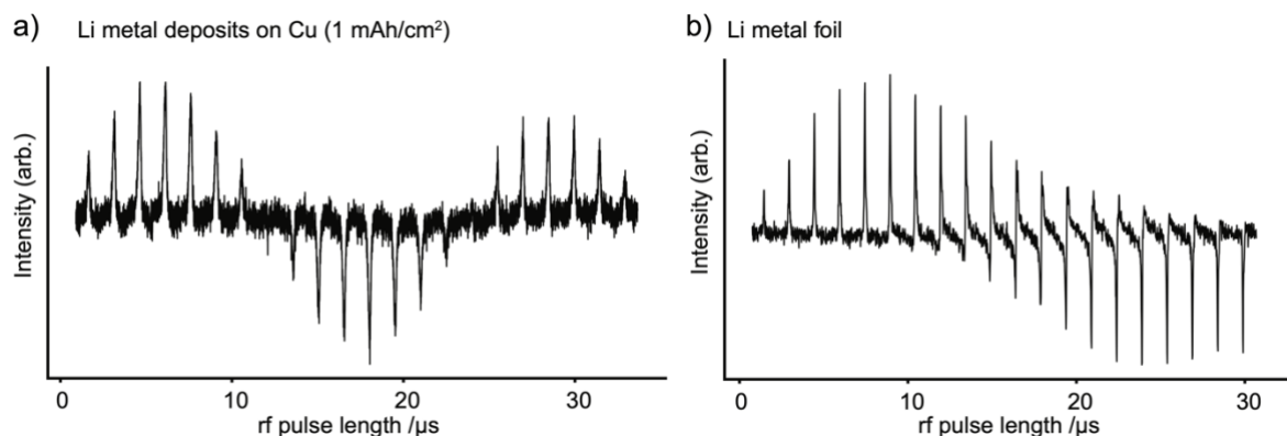
Figure S1. Experimental nutation curves of a) the Li deposits on Cu ( 1 \text{ mAh/cm}^2 ) nutate sinusoidally as expected for samples that do not experience skin depth issues. b) The pristine Li metal foil nutates in a more complex way due to skin depth effects.
