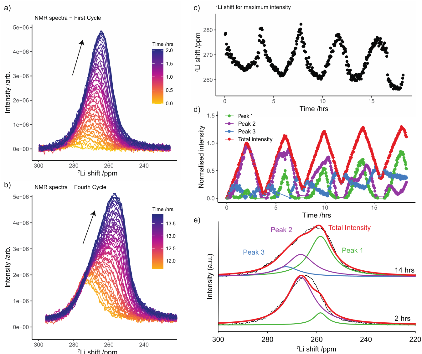
Figure S14. ^7\text{Li} metal shift in in DOL/DME electrolyte. a) The Li metal spectra during charge (plating) in the first cycle. b) The Li metal spectra during charge (plating) in the fourth cycle. c) The ^7\text{Li} shift of the maximum intensity of the Li metal resonance during cycling. d) The deconvoluted intensities of the Li metal spectra during cycling. e) An example of the fitted spectra at the end of charge in first and fourth cycle.
