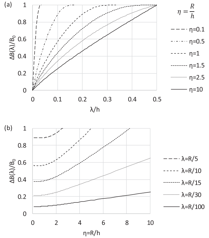
Figure 3. (a) The dependence of the decay of trapped field due to current redistribution on penetration depth \lambda for different values of the bulk superconductor aspect ratio \eta = R/h . (b) The decay of trapped field as a function of aspect ratio for different values of penetration depth.
