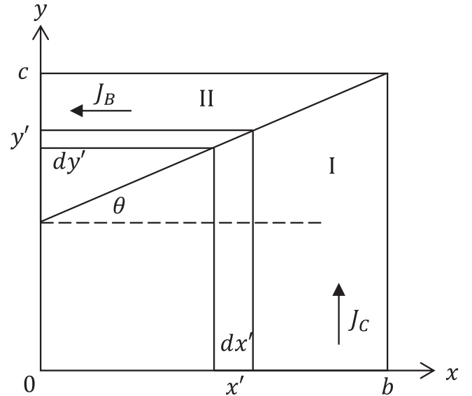
Figure 5. Illustration of the schematic of integration. The surface element is x'dy' + y'dx' (the area of the 'L'-shaped region) and the integration limits are x' = 0 and x' = b .
