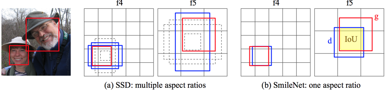
Figure 3. Example of matched default box for the face confidence heatmaps C_{f[4:5]} , produced by f4 and f5 output convolution layers (see Fig. 2). (a) Dotted boxes (grey) represent multiple candidate default boxes with different aspect ratios. In this case, when calculating the regression loss of the bounding box in the process of SmileNet training, the various shapes of the matched default box (blue) do not help converge the solution. Thus, (b) SmileNet uses only one aspect ratio in the matching process of the default box d . The example image is one of the sample images of AFLW dataset [12].
