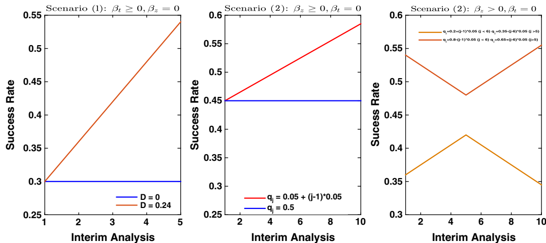
FIGURE 1 The per block success rate under different time trend assumptions, plotted over time. Left plot corresponds to scenario 1 (changes in standard of care), and middle and right plots correspond to different cases of scenario 2 (patient drift)
