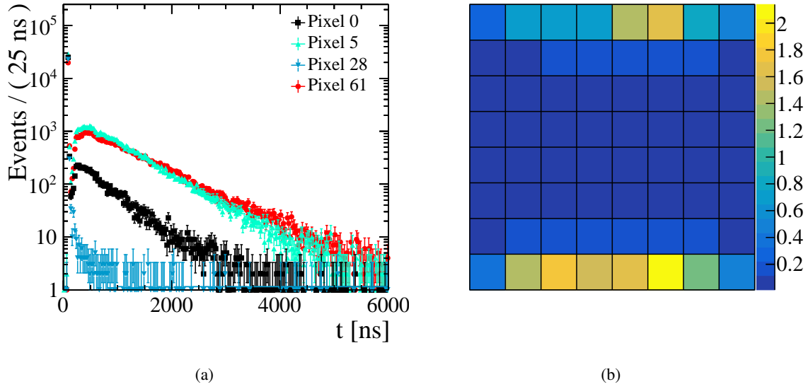
Figure 7. (a): time-spectra in logarithmic vertical scale for four pixels of tube FB4439. (b): map of the mean number of SIN pulses ( \mu_{\text{SIN}} ) for all the pixels of tube FB4439 (pixel-0 is top-left, pixel-7 is top right and pixel-63 is bottom-right).
