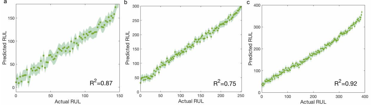
FIG. 4. Remaining useful life prediction without definite knowledge of the temperature.
