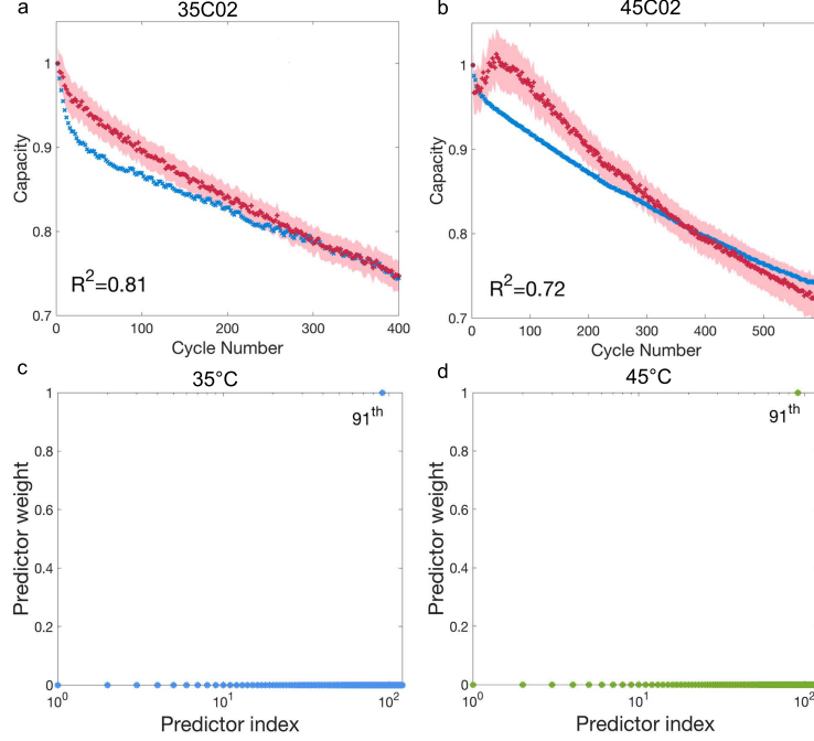
FIG. 3. Capacity estimation without definite knowledge of the temperature. The curves show the estimated (red) and measured (blue) capacity for cell cycled at (a) 35°C and (b) 45°C; the cycling temperature is not an input to our model. The shaded area indicates \pm 1 standard deviation. Both EIS spectra are collected at the state V (15 minutes resting after fully charging). R^2 is shown on the left bottom in each panel. ARD shows that the EIS-capacity GPR models at 35°C (c) and 45°C (d) assign the largest weight to the 91 st feature with the corresponding frequency of 17.80 Hz. The irrelevant features have weights close to zero.
