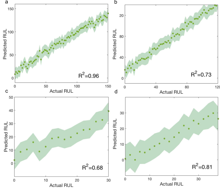
FIG. 2. Predicting remaining useful life. The predicted RUL of 25C05-25C08 testing cells (a-d) cycled at 25°C (shown as green curves). The end of life (EoL) of these four testing cells is 150, 120, 30 and 38, respectively, which is defined as the cycle number when the capacity drops below its initial 80%. The testing EIS spectra are collected at the state V (15 minutes resting after fully charging). The shaded region indicates \pm 1 standard deviation. R^2 is shown on the right bottom in each panel.
