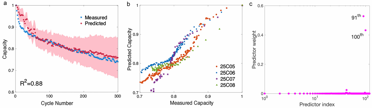
FIG. 1. Estimating battery capacity. (a) Estimated (red curve) and measured (blue curve) capacity as a function of cycle number for the 25C05 cell. The coefficient of determination ( R^2 ) of this model is shown on the left bottom. (b) The measured capacity against the estimated capacity of all four testing cells cycled at 25°C. The capacity is normalised against the starting capacity in each case. (c) ARD shows that the impedance at low frequency is most correlated with degradation. The pink points correspond to the 120 frequencies in the range of 0.02 Hz-20 kHz. The GPR model assigns the largest weights to the 91 st and 100 th features, corresponding to 17.80 and 2.16 Hz, respectively. The less relevant features have weights close to zero.
