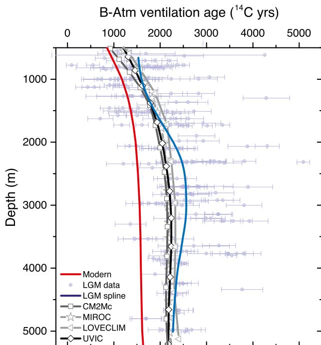
Figure 8. A compilation of Last Glacial Maximum (LGM) modeled global average radiocarbon activity (lines with open symbols; Chikamoto, Abe-Ouchi, et al., 2012; Chikamoto, Menviel, et al., 2012; Menviel et al., 2017; Muglia et al., 2018; Galbraith & de Lavergne, 2019) and reconstructed radiocarbon activity (light blue crossed circles, with 1 sigma error bars; Skinner et al., 2017), expressed relative to the atmosphere and as a function of water depth. A cubic spline fit to the proxy data (solid blue line), and the modern radiocarbon profile corrected for the influence of nuclear bomb testing in the twentieth century (solid red line; Key et al., 2004), are shown for comparison. The ocean is generally observed, and modeled, to have been more radiocarbon depleted at the LGM, relative to the contemporary atmosphere, as compared to modern, with generally good agreement between models despite a slight underestimation of simulated radiocarbon ventilation ages in the middepth ocean, where a “bulge” in ventilation ages is apparent (Burke et al., 2015; Skinner et al., 2017).
