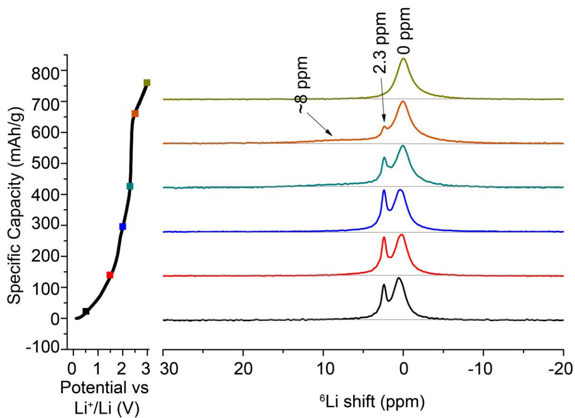
Figure 6. ^6\text{Li} NMR spectra of \text{VS}_4\text{-GO} during charge. The dashed baseline is shown so that the broader resonance at ~8 ppm can be seen more clearly.
