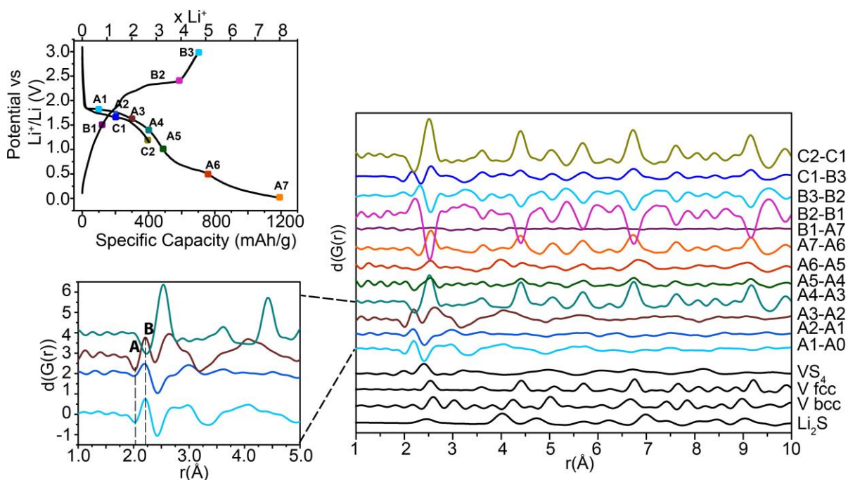
Figure 9. Ex-situ Pair Distribution Function data of \text{VS}_4 -rGO samples. The simulated PDF patterns of the model compounds ( \text{VS}_4 , \text{Li}_2\text{S} , bcc and fcc V) are given at the bottom. The vertical lines correspond to fcc-V
