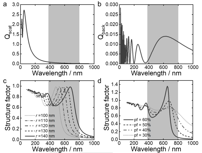
Figure 3. (a) Total scattering cross section of a Mie sphere ( r = 140 nm, n_{pore} = 1.33 , n_{matrix} = 1.5 ). (b) Backscattering cross section of the same Mie sphere. (c) Percus-Yevick structure factor for a packing fraction ( pf ) of 50%, with n_{pore} = 1.33 , n_{matrix} = 1.5 and varying radius. (d) Structure factor for r = 140 nm and varying pf . The grey band indicates the wavelength range in Figure 2.
