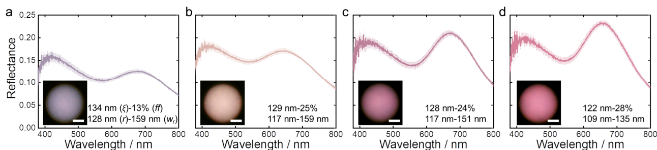
Figure 4. Reflectance spectra and microscope images (inset) for CLEG4 microspheres prepared in different conditions to enhance the contribution of the first structural peak towards a purer red color. The evaporation temperature and macromonomer loading are: (a) 60 °C with no NB-PCL; (b) 60 °C with 20% NB-PCL; (c) 65 °C with 25% NB-PCL; (d) 65 °C with 30% NB-PCL. The correlation length ( \xi ), filling fraction ( ff ), pore radius ( r ), and pore size distribution ( w_r ) determined from structural analysis are also stated. Scale bar for insets is 20 \mu m.
