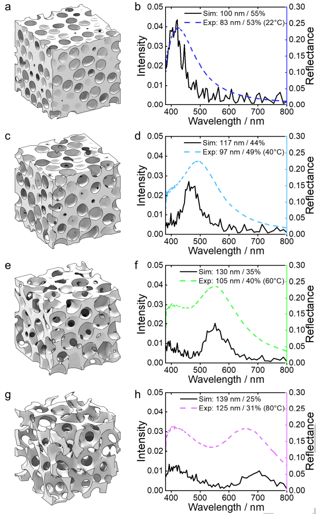
Figure 2. Finite difference time domain (FDTD) simulations on in silico synthesized foam structures: (a,c,e,g) Two-phase 3D models representing the photonic structures with different correlation lengths ( \xi_{sim} ) and filling fraction ( ff_{sim} ). The structural parameters of each structure, denoted \xi_{sim} / ff_{sim} are: (a) 100 nm / 55%, (c) 117 nm / 44%, (e) 130 nm / 35%, (g) 139 nm / 25%; (b,d,f,h) Simulated optical response (left axis; black solid lines) for these in silico synthesized structures and experimental spectra (right axis; colored dash lines) measured for photonic pigments prepared at 22, 40, 60 and 80 °C (from top to bottom).
