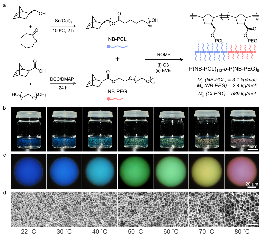
Figure 1. (a) Schematic of the synthetic route for the biocompatible BBCP, including preparation of the two macromonomers, NB-PCL and NB-PEG, and their copolymerization via ring-opening metathesis polymerization (ROMP) to form \text{P}(\text{NB-PCL})\text{-}b\text{-P}(\text{NB-PEG}) ; the number averaged molecular weights ( M_n ) are also included. (b) Photographs recorded under direct illumination of aqueous dispersions of photonic BBCP pigments, formed from the controlled evaporation of monodisperse toluene/water microdroplets at different temperatures ( T = 22\text{--}80^\circ\text{C} ). (c) Corresponding micrographs of individual BBCP microspheres for each temperature, showing the rainbow of colors. (d) Cross-sectional SEM micrographs reveal the internal porous nanoarchitecture of this series of photonic pigments.
