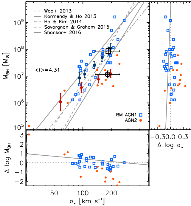
Figure 2. The M_{\text{BH}}-\sigma_* plane for local samples of RM AGN1 (blue open squares) and AGN2 (red filled circles), together with average M_{\text{BH}} of the RM AGN1 (dark blue) and AGN2 (dark red), computed in (not independent) bins of stellar velocity dispersion. The black open square (circle) shows the M_{\text{BH}} average value of the RM AGN1 (AGN2) sample in the 135 < \sigma_* < 250 \text{ km s}^{-1} stellar velocity bin and has been plotted at the position of the average \sigma_* . Some relations from literature are also reported (see the text for details). Bottom: residuals of M_{\text{BH}} with respect to the relations of Woo et al. (2013, dotted grey line) and Kormendy & Ho (2013, solid line). Right: same as bottom panel but for \sigma_* .
