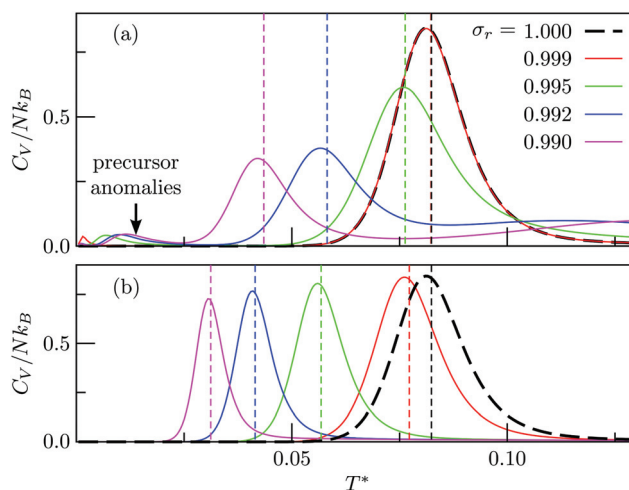
Fig. 6 Heat capacity of doped LJ_{75} clusters for different values of \sigma_r , calculated using either (a) all local minima or (b) just bimimima. Dashed vertical lines mark the value of T_s^* calculated using (7).
