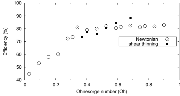
Figure 4. Efficiency : proportion of total ejected ink within the main drop.
