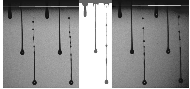
Figure 5. Comparison for 1000 ppm PS210 in DEP.
