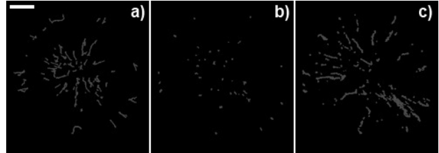
Figure 5. Particle trajectories for 10% v ethylene glycol-water containing 0.01% v 620 nm spheres. a) Motion of particles was initially relatively fast towards the contact line (0–1 s). b) Radial motion slowed as ethylene glycol became the main component (1–2 s). c) Radial motion during remainder of drying (2 s onwards). The scale bar is 20 \mu m.
