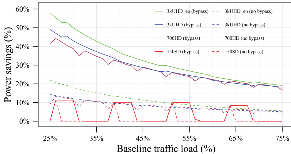
Figure 7.8: Power savings achieved by optically bypassing popular TV channels in the network core, as a function of the baseline traffic load in the node
