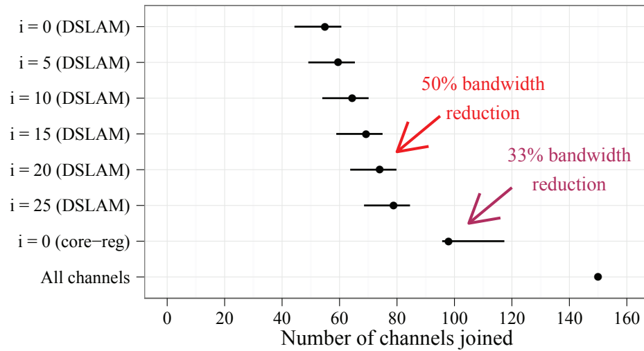
Figure 6.3: Number of channels joined when using the selective joining scheme for various values of the inactive set size
