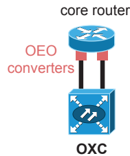
Figure 7.7: Hybrid node
