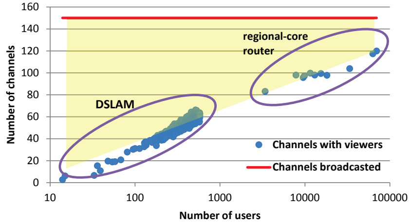
Figure 6.1: Average number of active channels (TV channels with viewers) per network node (including DSLAMs and core-regional routers). Nodes are ordered by the number of users they serve
