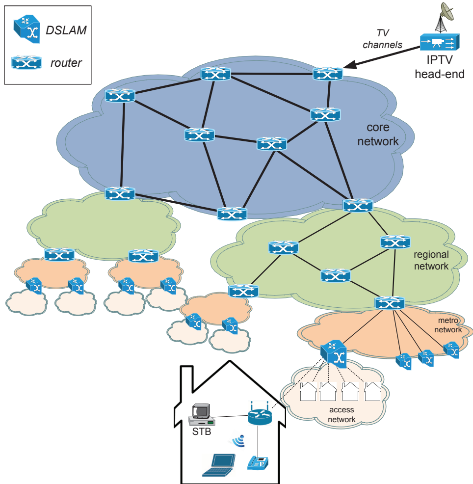
Figure 2.5: IPTV reference architecture
