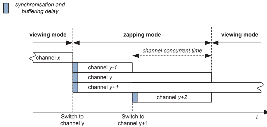
Figure 5.2: Predictive pre-joining of TV channels
