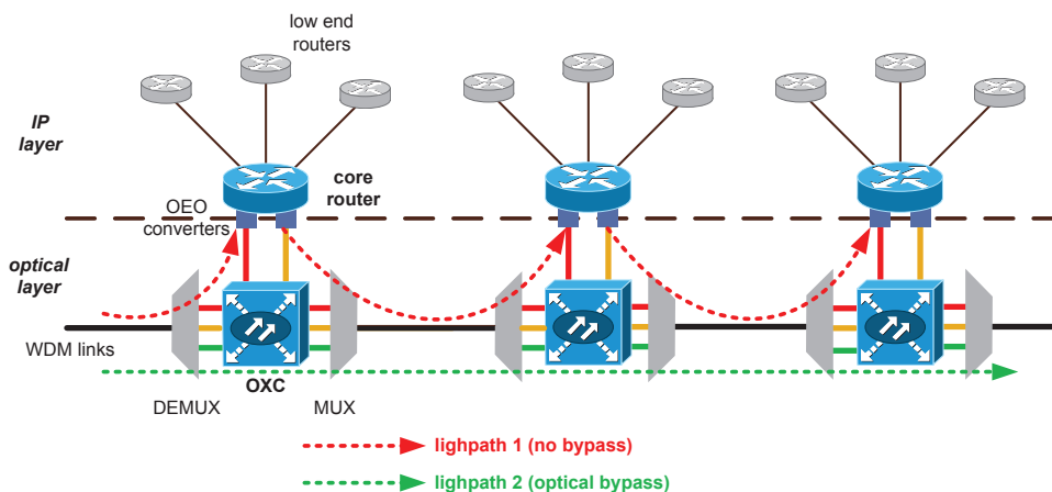
Figure 7.2: Optical network employing optical bypass techniques
