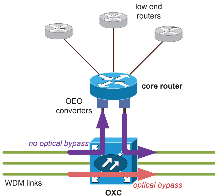
Figure 3.2: Optical bypass-enabled network node
