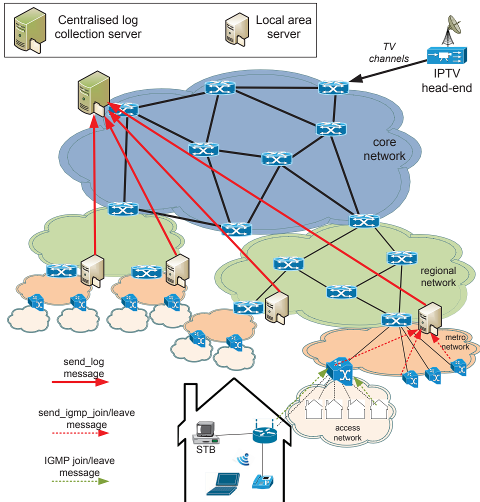
Figure 4.2: Data collection process
