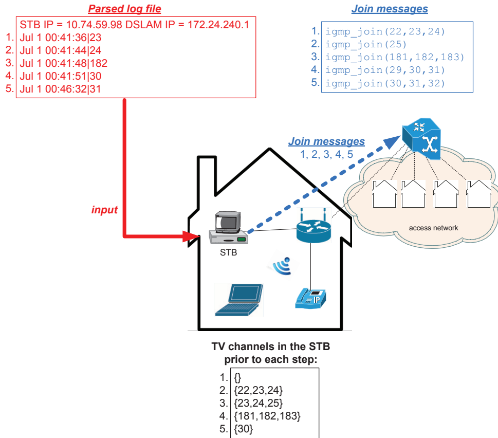
Figure 5.3: Proposed methodology
