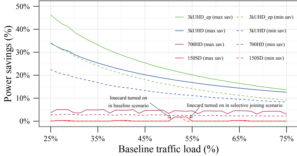
Figure 6.7: Power savings after introducing the proposed scheme as a function of the baseline traffic load in the node (regional network)
