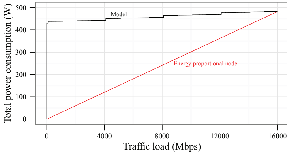
Figure 6.6: Current router power consumption vs energy-proportional node
