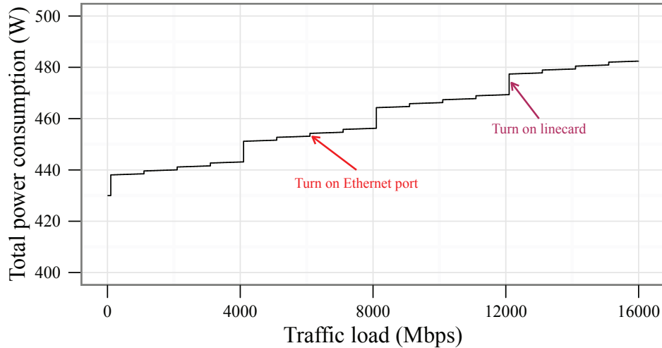
Figure 6.5: Power consumption model (zoomed)
