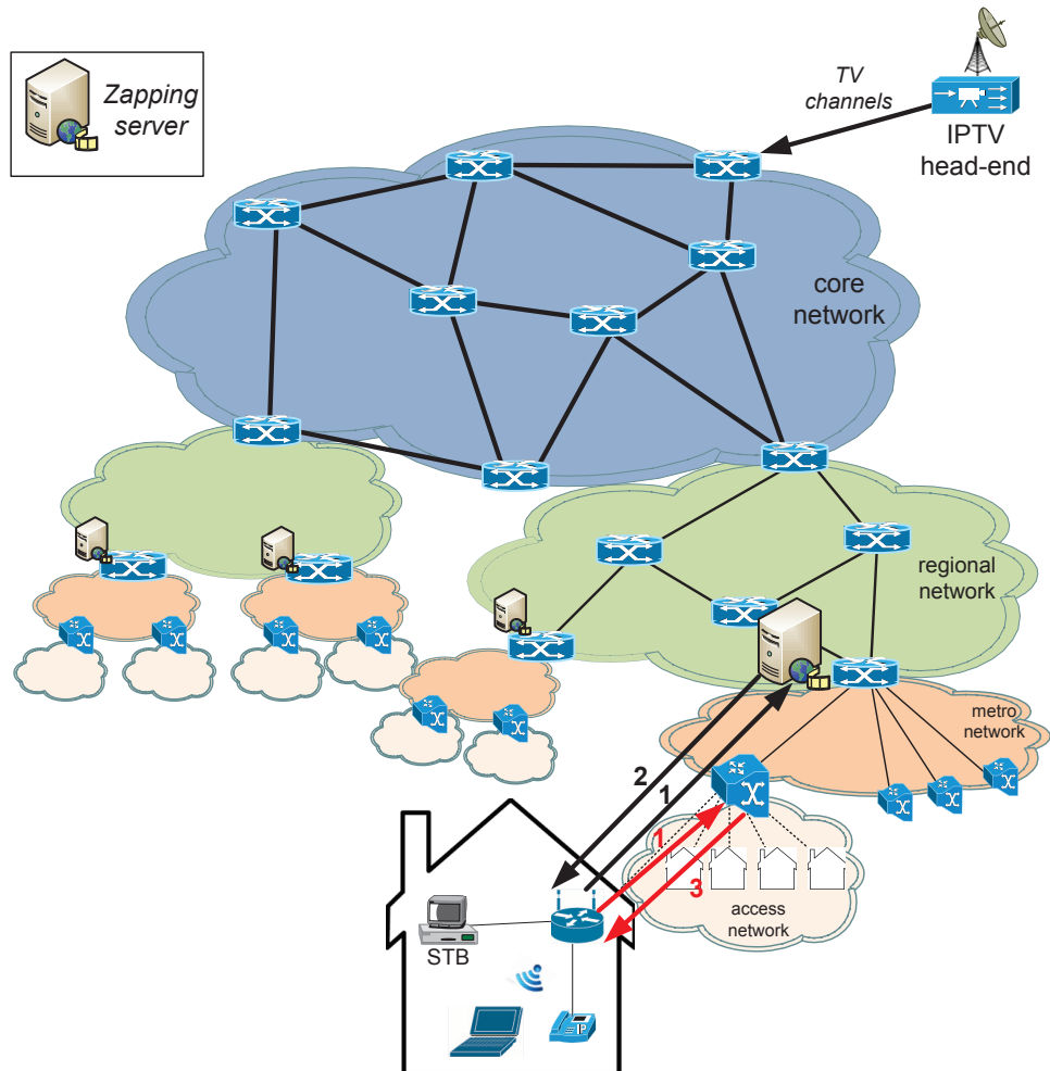
Figure 3.1: Zapping servers introduced in the IPTV network to mitigate the high channel change delay
