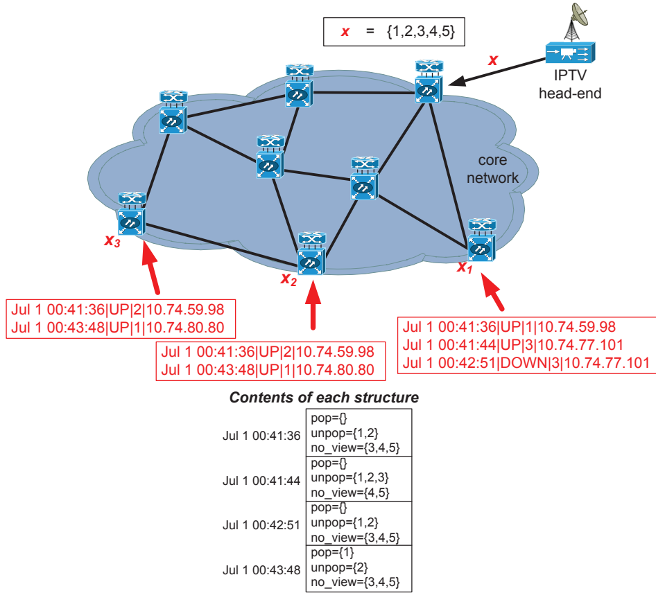
Figure 7.3: Proposed methodology
