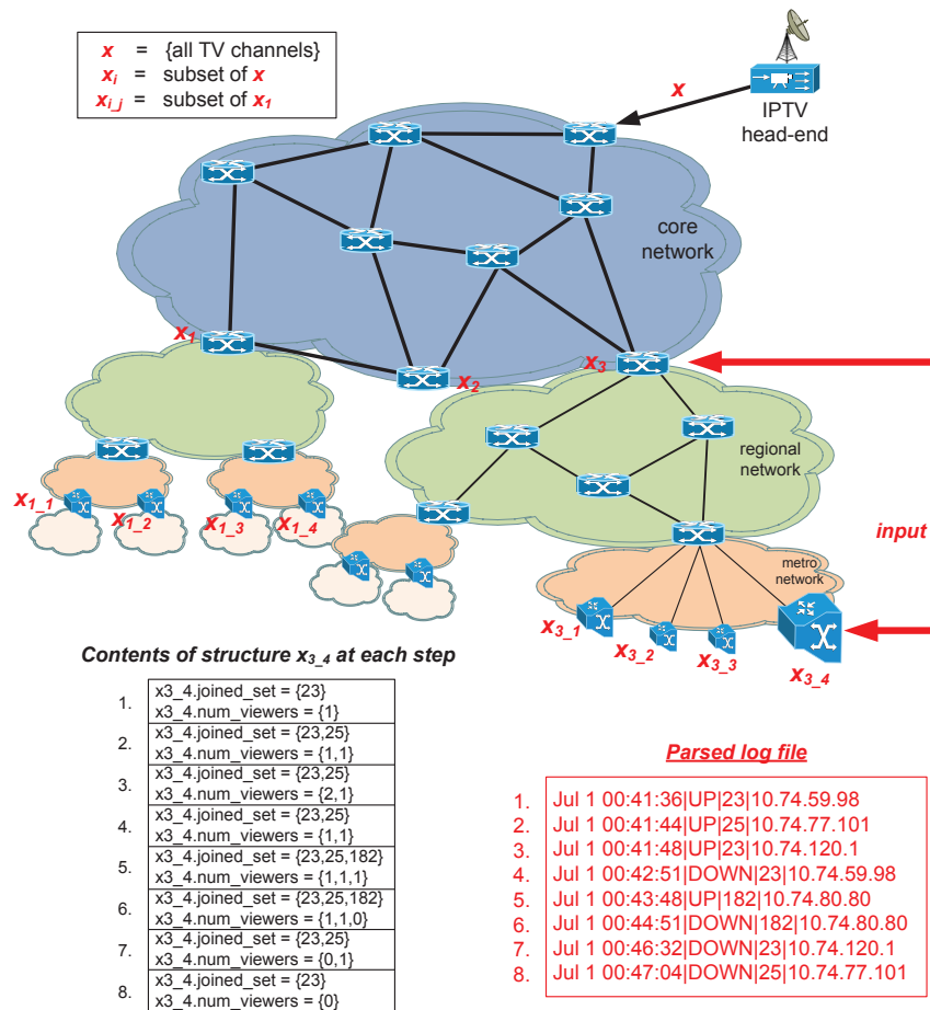
Figure 6.2: Proposed methodology
