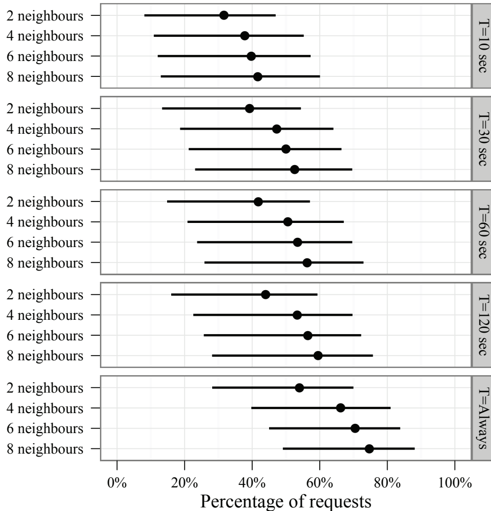
Figure 5.9: Variance of the percentage of requests that experience no delay by using the simple scheme for various values of channel concurrent time T and number of neighbours. In the graph the median, 5th and 95th percentile are presented
