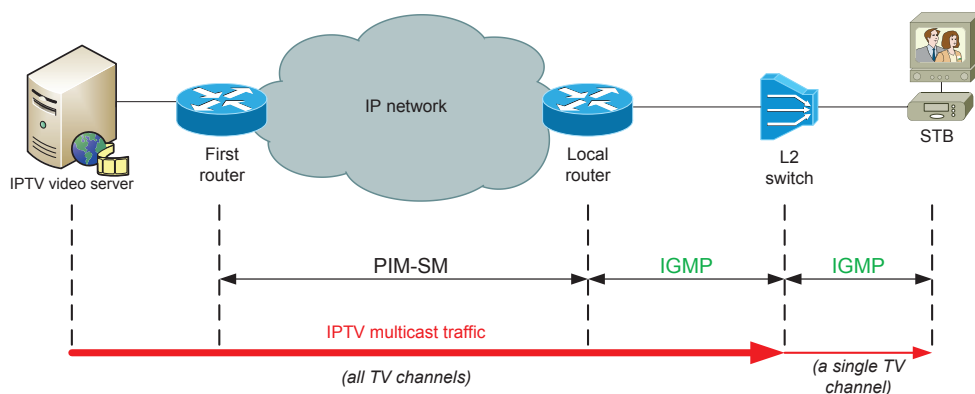
Figure 2.4: IGMP basic network architecture
