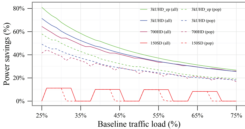
Figure 7.9: Power savings achieved by optically bypassing all TV channels in the network core (compared to popular TV channels only), as a function of the baseline traffic load in the node
