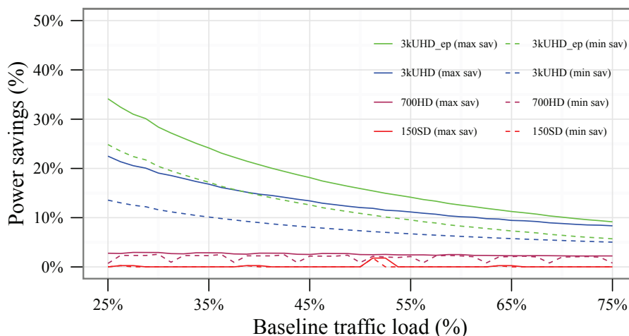
Figure 6.8: Power savings after introducing the proposed scheme as a function of the baseline traffic load in the node (core network)
