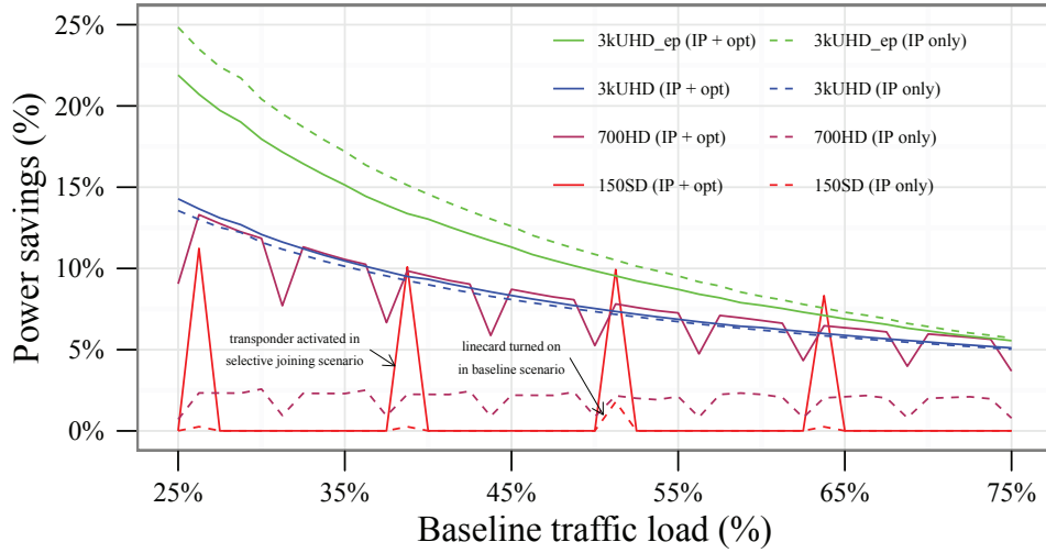
Figure 7.6: Power savings of using the selective joining scheme considering an optical IP network, as a function of the baseline traffic load in the node (core network)
