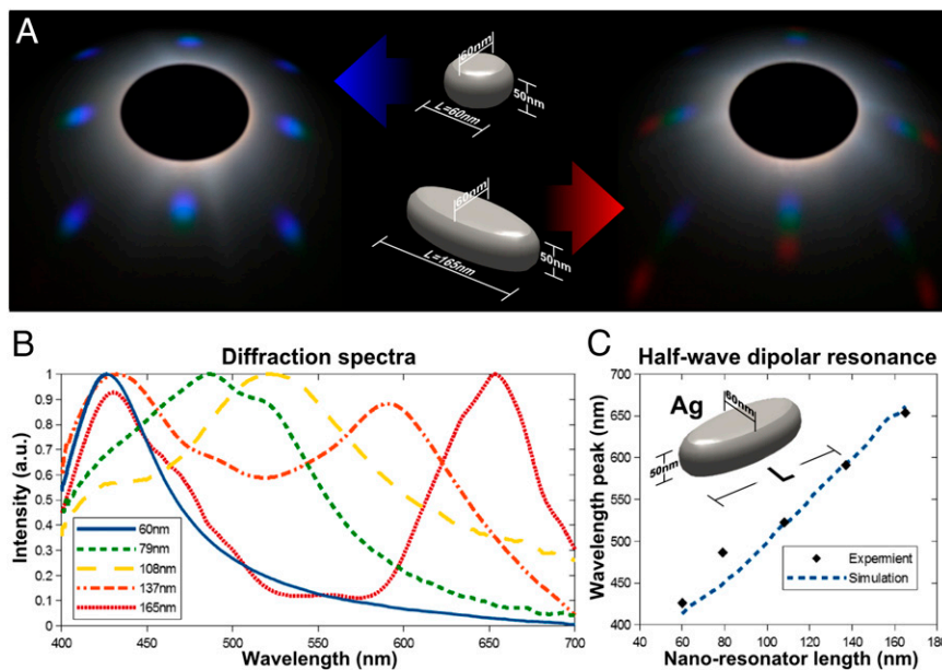
Fig. 1. Spectral characteristics of the scattering of silver nanoparticles. (A) Projected white light diffraction pattern produced by square grids of nanoparticles of 1- \mu m pitch. The diffracted light carries the scattering spectrum of the nanoparticle. (B) Measurement of the far-field spectra of nanoparticles of 60 nm in width, 50 nm high, and of multiple lengths. (C) Experimental and simulated plot of the half-wave dipolar resonance peak along the visible spectra.
