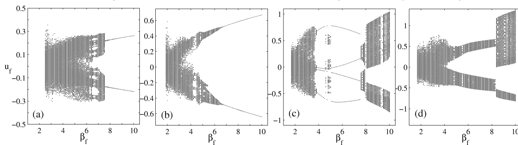
FIGURE 5. Bifurcation diagrams with flame aspect ratio, \beta_f = L_f/R , as control parameter at flame positions (a) x_f = 0.1 , (b) x_f = 0.2 , (c) x_f = 0.3 , and (d) x_f = 0.4 . \beta_f is varied by changing the mean flow velocity U_0 but keeping the equivalence ratio and flame speed constant. In all cases the initial condition is the steady unperturbed flame. Firstly, we see that periodic oscillations are not necessarily the preferred stable states; quasi-periodic and chaotic oscillations are seen over significant parameter ranges. Secondly, chaotic oscillations are seen in all cases at low aspect ratios.
