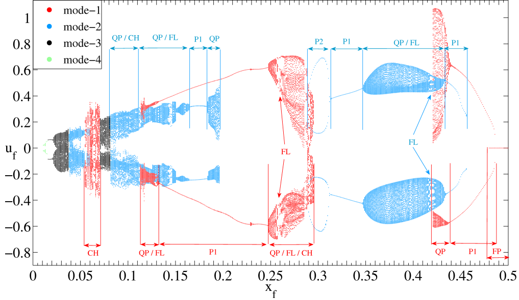
FIGURE 3. Bifurcation diagram with flame position, x_f , as control parameter keeping all other parameters constant: \phi_{mean} = 0.85 , \beta_f = L_f/R = 7 , ratio of combustion to acoustic time scales = L_f/ML_0 = 2.2 . The u_f values are the peaks and troughs of the time-series once the system has settled to its ultimate stable state. One set of points is obtained by increasing x_f starting from the stable state at the previous x_f . The other set of points is obtained by decreasing x_f . The different colours represent the most dominant acoustic mode in the power spectrum of the oscillation; mode-1 is shown in light grey (red online), mode-2 in dark grey (blue online), mode-3 in black (black online) and mode-4 in very light grey (green online). Some branches end abruptly because the state becomes unstable. The sequence of bifurcations are explained in the text. This chart shows that the system can have a stable fixed point (labelled FP), stable period-1 oscillations (labelled P1), period-2 oscillations (labelled P2), frequency-locked or period- k oscillations (labelled FL), quasi-periodic oscillations (labelled QP) and chaotic oscillations (labelled CH) depending on the x_f and initial conditions. There are several bi-stable regions, hence mode switching and hysteresis are possible.
