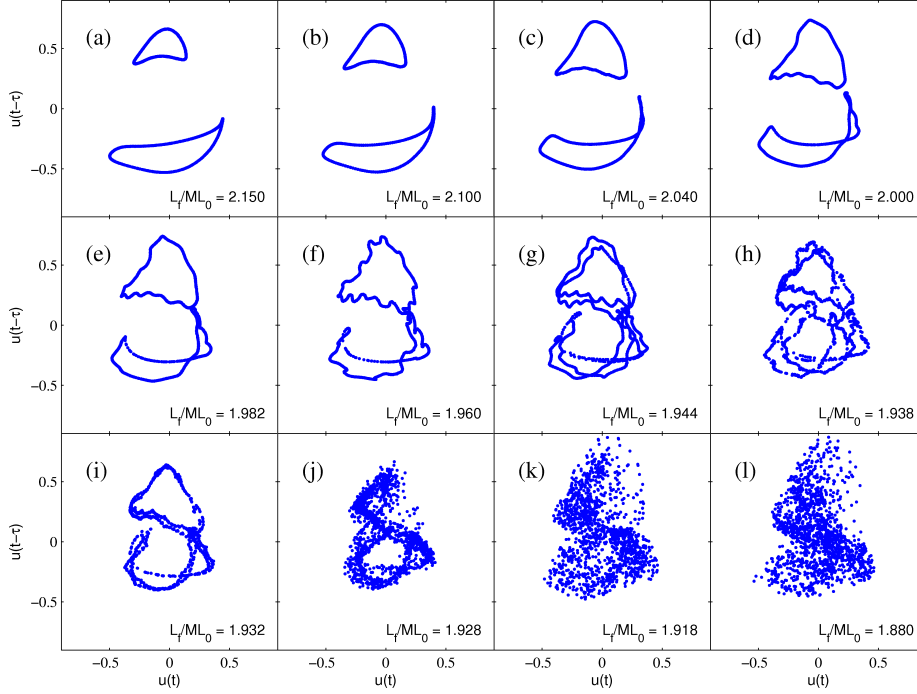
FIGURE 15. The Ruelle-Takens-Newhouse route to chaos observed in the L_f/ML_0 range of 1.88 to 2.15 ( x_f = 0.4 ). (a) to (l) show the Poincaré sections of phase portraits of the final state of the system at each operating point (varying L_f/ML_0 ). The stable quasi-periodic state (2-torus) in (a) develops corrugations on its surface due to stretching and folding (see sub-figures (c), (d), (e) and (f)). This is followed by torus breakdown (see sub-figures (g), (h) and (i)) to chaos (sub-figures (j), (k), (l)).
