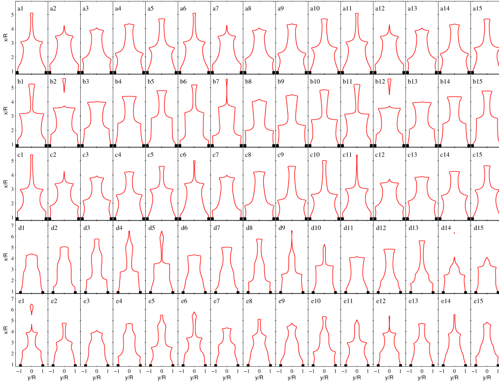
FIGURE 7. Instantaneous flame images of the self-excited flame for different types of oscillation: (a) period-1 oscillation at x_f = 0.435 (mode-2 branch) (b) period-2 oscillation at x_f = 0.3 , (c) quasi-periodic oscillation at x_f = 0.4 , (d) period- k oscillation at x_f = 0.286 and (e) chaotic oscillation at x_f = 0.4 . For (a) to (d) all other parameters are the same as in figure 8, while (e) has the same parameters as figure 11(e). 15 images are shown for each case spanning 3 cycles of the dominant frequency.
