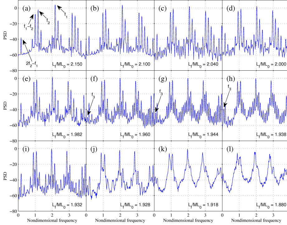
FIGURE 16. The Ruelle-Takens-Newhouse route to chaos observed in the L_f/ML_0 range of 1.88 to 2.15 ( x_f = 0.4 ). (a) to (l) show the power spectra of the velocity at the flame position for these states (corresponding to the same subfigures in figure 15). The power spectral density is on a logarithmic scale.
