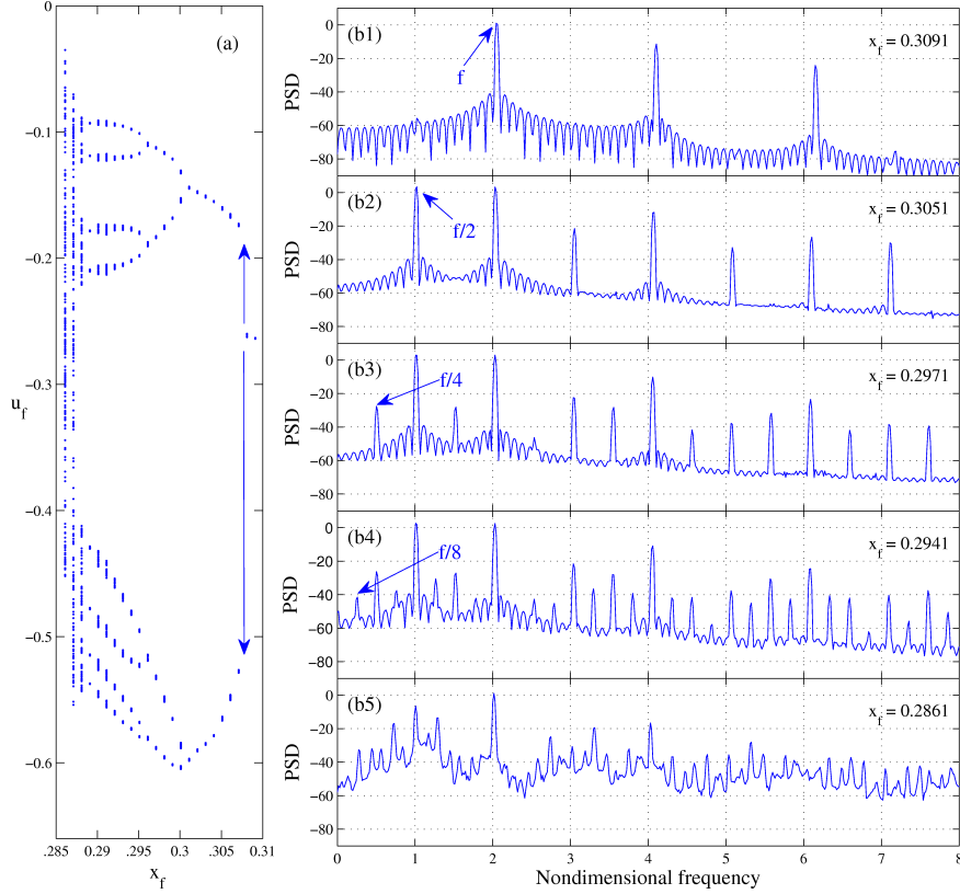
FIGURE 14. The period doubling route to chaos observed in the x_f range of 0.285 to 0.31 ( L_f/ML_0 = 2.0 ) (a) Bifurcation diagram constructed using the troughs of the time series of velocity perturbations at the flame position, u_f . A series of period doubling bifurcations occur at x_f = 0.307 (period 1 to 2), x_f = 0.301 (period 2 to 4) and x_f = 0.296 (period 4 to 8). (b) Power spectra of velocity at the flame showing the emergence of subharmonics ( f/2 (figure (b2)), f/4 (figure (b3)), f/8 (figure (b4))) at the above mentioned values of x_f , finally leading to chaotic oscillations at x_f = 0.288 (figure (b5)). The power spectral density is on a logarithmic scale.
