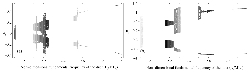
FIGURE 6. Bifurcation diagrams with non-dimensional fundamental frequency of the duct as control parameter at positions x_f = 0.07 in (a) and x_f = 0.4 in (b). The non-dimensional frequency is varied by changing the duct length L_0 but keeping all other parameters constant. Note that the ratio of combustion to acoustic time scales, L_f/ML_0 , varies when L_0 changes. In all cases the steady state flame position is used as the initial condition for the simulation.
