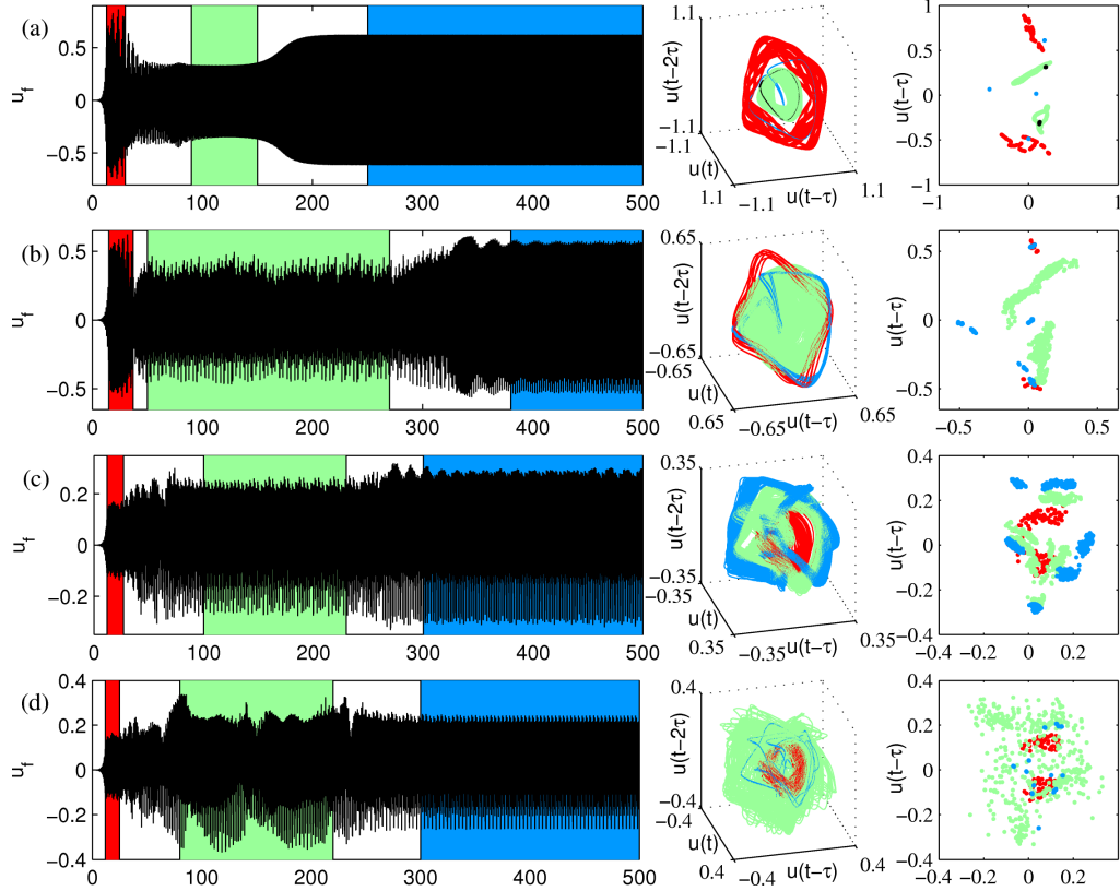
FIGURE 13. A continuation of the previous figure, this figure also shows the intermediate states in the time evolution of the self-excited system: (a) x_f = 0.295 , L_f/ML_0 = 2.2 , (b) x_f = 0.2862 , L_f/ML_0 = 2.0 , (c) x_f = 0.066 , L_f/ML_0 = 2.2 , and (d) x_f = 0.063 , L_f/ML_0 = 2.2 . The windows of the time series that are used to extract the phase portraits are shown as coloured patches. Intermediate states are shown in red and green, and the ultimate stable state is shown in blue.
