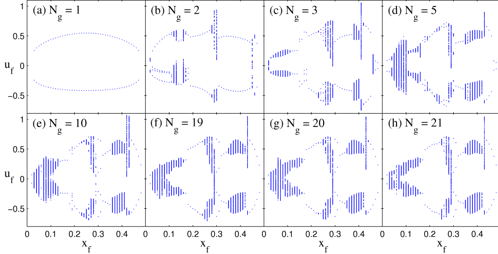
FIGURE 4. Bifurcation diagrams with flame position, x_f , as control parameter with different numbers of Galerkin modes, N_g , in the discretization: (a) N_g = 1 , (b) N_g = 2 , (c) N_g = 3 , (d) N_g = 5 , (e) N_g = 10 , (f) N_g = 19 , (g) N_g = 20 and (h) N_g = 21 . All other parameters are kept constant: \beta_f = L_f/R = 7 , ratio of combustion to acoustic time scales = L_f/ML_0 = 2.2 . At a given value of x_f the points on the diagrams are the peaks and troughs of the velocity time series data once the system has reached a stable state. (a) shows that for N_g = 1 the system always reaches a period-1 limit cycle. As the number of modes is increased, even though the higher modes are more heavily damped, modal interactions result in non-harmonic states such as period-2, period- k and quasi-periodic states. Further, the maximum amplitudes of oscillations are significantly higher than the single-mode case (a). Comparing (f), (g) and (h) shows that the solutions are nearly independent of the discretization when N_g is sufficiently large.
