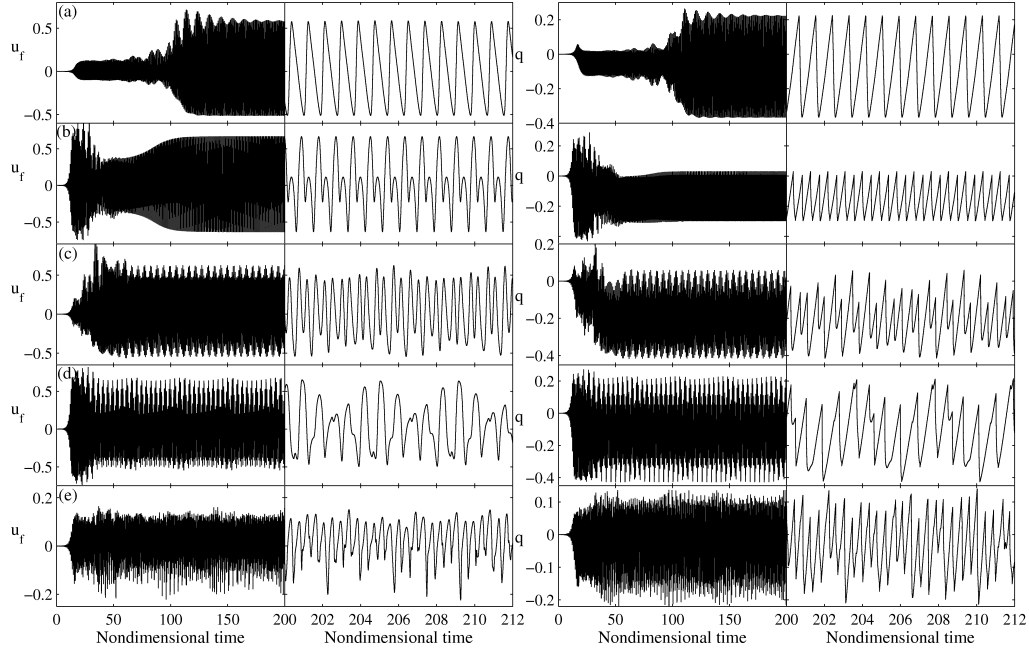
FIGURE 8. Time series of velocity and heat release rate for the different types of oscillation corresponding to different flame positions of figure 3: (a) period-1 oscillation at x_f = 0.45 , (b) period-2 oscillation at x_f = 0.3 , (c) quasi-periodic oscillation at x_f = 0.4 , (d) period- k oscillation at x_f = 0.286 and (e) chaotic oscillation at x_f = 0.046 .
