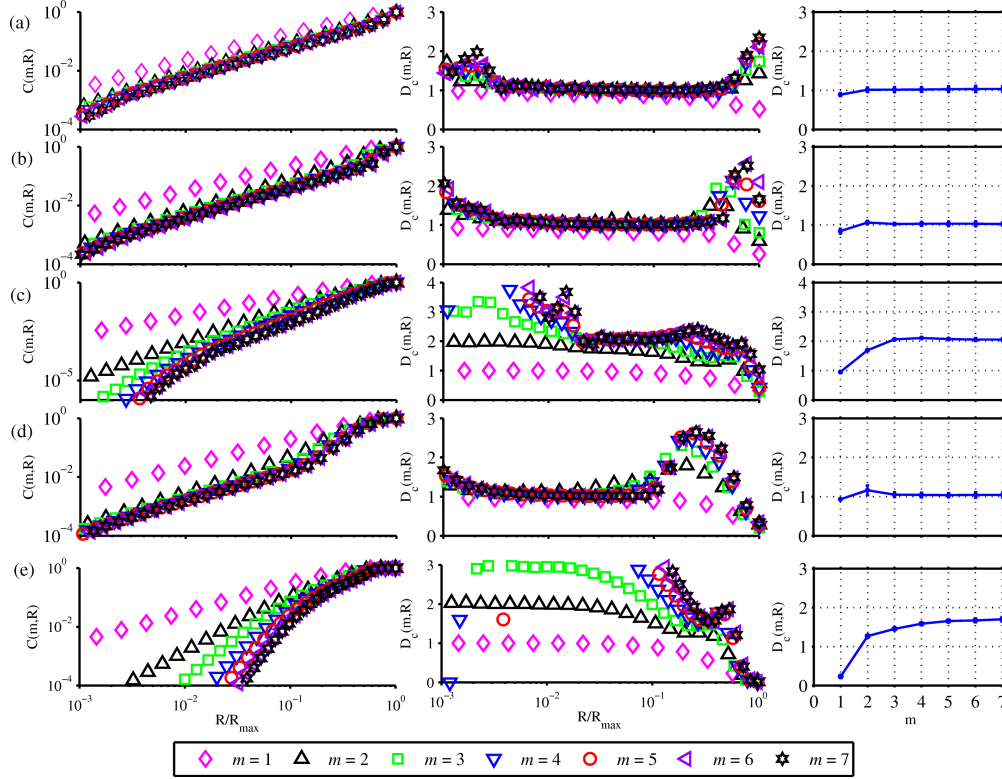
FIGURE 11. This figure shows the correlation sum, C(m, R) (left column), and its local slope, D_c(m, R) = \partial \log C(m, R) / \partial \log R (middle column), as functions of the Euclidean distance, R/R_{max} , for an embedding dimension up to m = 7 . Shown in the right column is the correlation dimension defined as the average slope ( \bar{D}_c(m, R) = \partial \log C(m, R) / \partial \log R ), over the range of radii where the slope remains fairly constant, as a function of the embedding dimension, m . (a) to (e) correspond to period-1, period-2, quasi-periodic, period- k and chaotic oscillations of figure 8.
