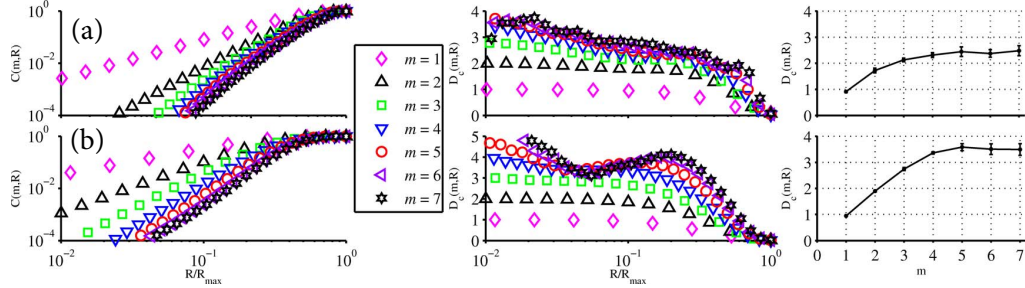
FIGURE 17. This figure shows the correlation sum, C(m, R) (left column), and its local slope, D_c(m, R) = \partial \log C(m, R) / \partial \log R (middle column), as functions of the Euclidean distance, R/R_{max} , for an embedding dimension up to m = 7 . Shown in the right column is the correlation dimension defined as the average slope ( \overline{D_c(m, R)} = \partial \log C(m, R) / \partial \log R ), over the range of radii where the slope remains fairly constant, as a function of the embedding dimension, m . (a) chaotic oscillations in the period-doubling route to chaos, figure 14(b5) (b) chaotic oscillations in the Ruelle-Takens-Newhouse route to chaos, figure 15(1).
