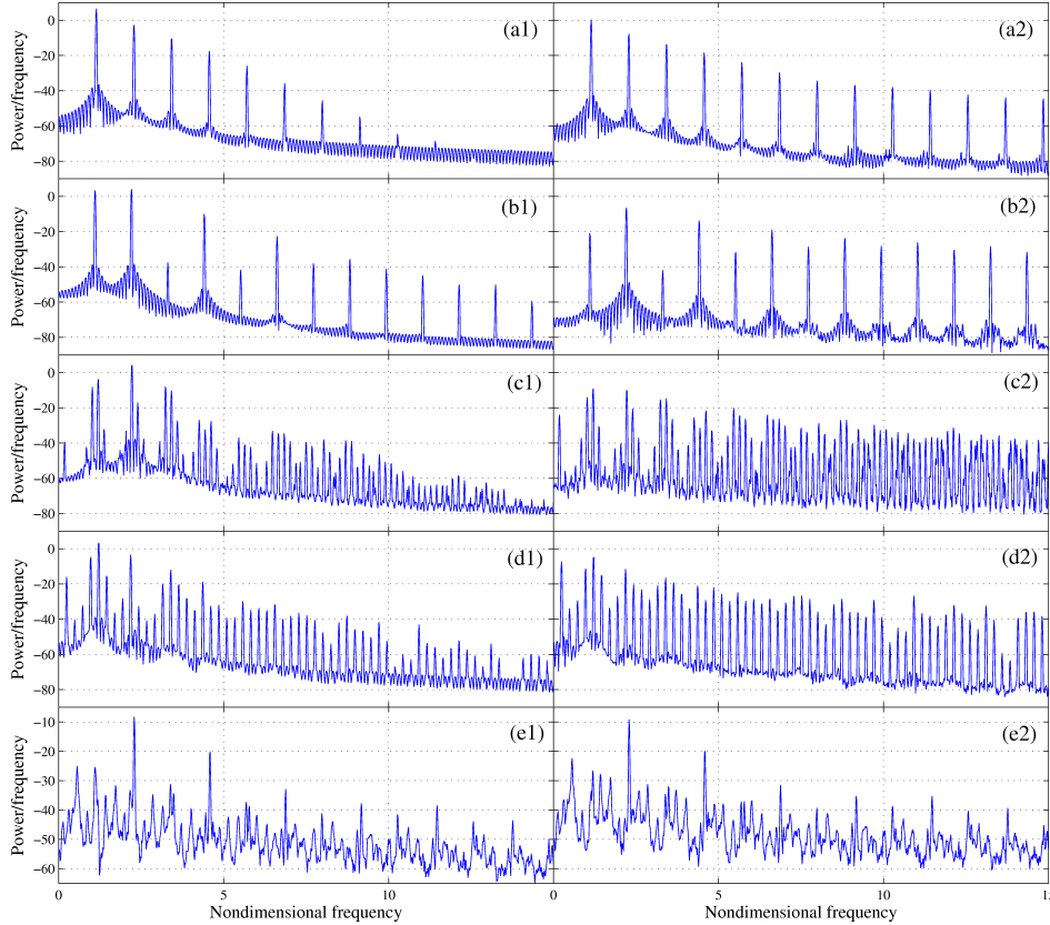
FIGURE 9. Power spectra of velocity (labelled 1) and heat release rate (labelled 2) for the different types of oscillation corresponding to different flame positions of figure 3: (a) period-1 oscillation at x_f = 0.45 , (b) period-2 oscillation at x_f = 0.3 , (c) quasi-periodic oscillation at x_f = 0.4 , (d) period-5 oscillation at x_f = 0.286 and (e) chaotic oscillation at x_f = 0.046 . The power spectral density is on a logarithmic scale.
