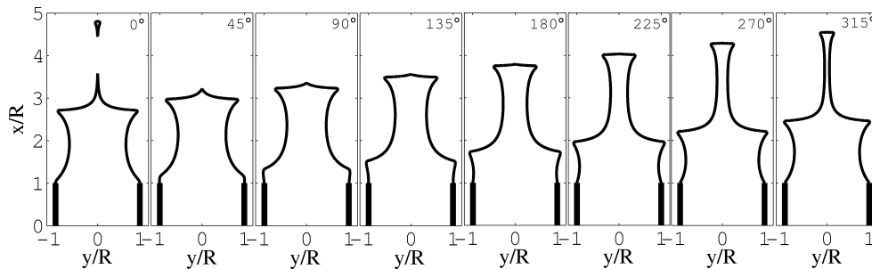
FIGURE 2. Instantaneous images of the flame during a period-1 limit cycle oscillation, mean equivalence ratio = \phi = 0.85 , ratio of flame height ( L_f ) to flame radius ( R ) = \beta_f = 5 . Note the formation of sharp cusps towards the products and flame pinch-off, which are characteristics of premixed flames seen in experiments (Baillot et al. 1992; Ducruix et al. 2000; Durox et al. 2005; Birbaud et al. 2006; Karimi et al. 2009)
