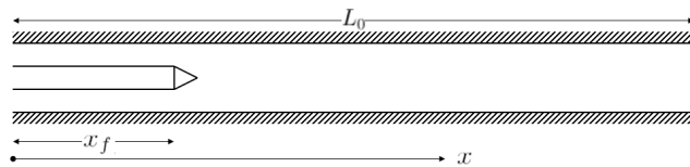
FIGURE 1. Diagram of the two-dimensional slot stabilized premixed flame in a duct. L_0 is the length of the duct, \tilde{x}_f is the flame position along the duct, \alpha = 0.2 is the fraction of the duct cross-sectional area occupied by the burner and the flow is from left to right.
