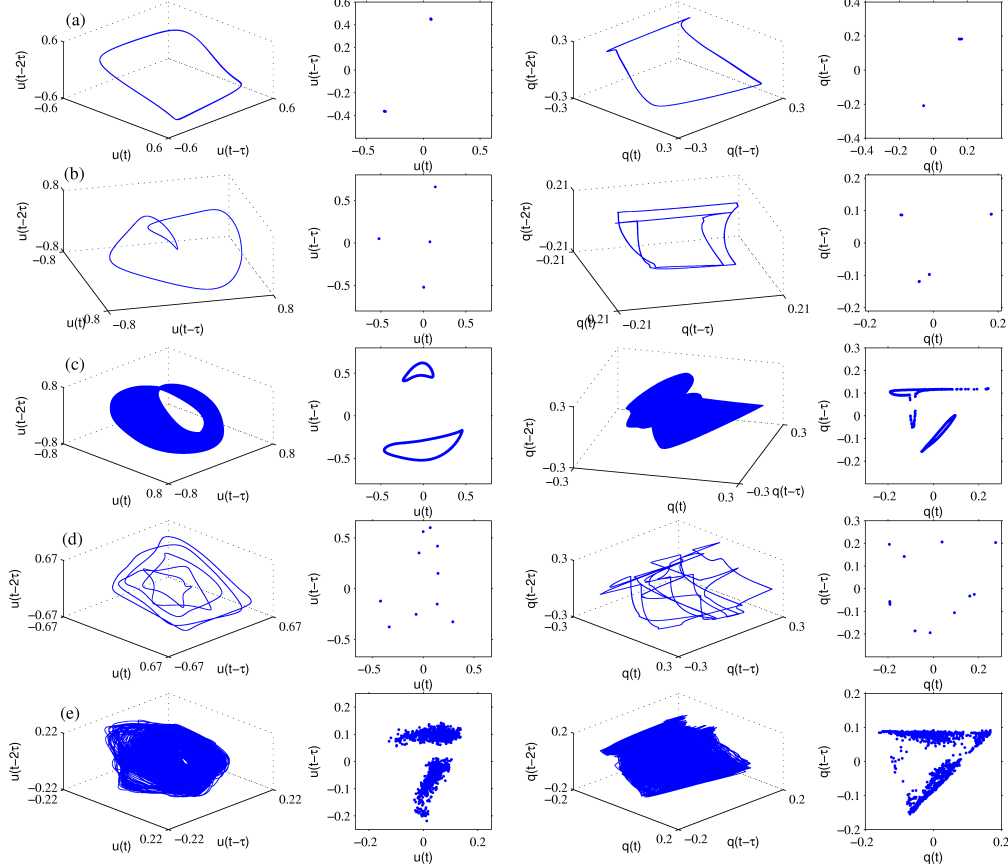
FIGURE 10. Phase portraits and Poincaré sections of velocity and heat release rate for the different types of oscillation corresponding to different flame positions of figure 3: (a) period-1 limit cycle oscillation at x_f = 0.45 , (b) period-2 oscillation at x_f = 0.3 , (c) quasi-periodic oscillation at x_f = 0.4 , (d) period- k oscillation at x_f = 0.286 and (e) chaotic oscillation at x_f = 0.046 .
