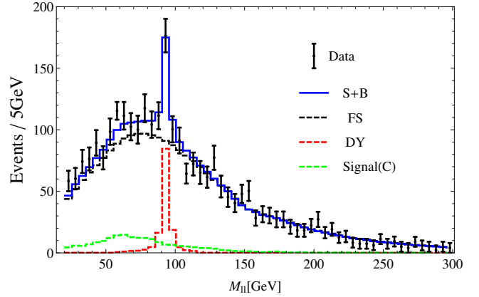
FIG. 1. Di-lepton invariant mass spectrum of CMS \ell^+\ell^-jj\cancel{E}_T events: expected non-DY background (black histogram), expected DY (red histogram), expected signal for benchmark C (green histogram) and expected signal plus background for benchmark C (blue histogram). 21 signal events are expected for m_{\ell\ell} > 100 \text{ GeV} , which is compatible with CMS data.
