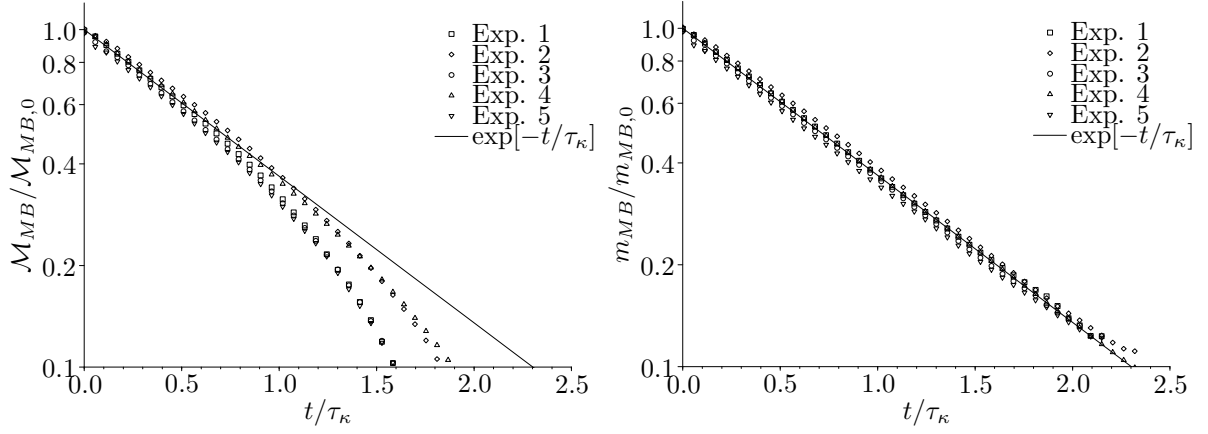
Figure 6: Evolution of the normalised quantity of dye m_{MB}/m_{MB,0} on a logarithmic axis with non-dimensional time t/\tau_\kappa . The time scale \tau_\kappa = V_0/(\kappa A_m) is the characteristic time for the convective mass transfer. We plot the ensemble-averaged data of the drops for each experiment using different symbols (see tables 4 and 5). The solid lines represent the exponential decrease predicted by the Newton-cooling model (13). In (a) we show the data before correction for the dye invisible to our detection system (see (59)), in (b) we show the data after correction according to (61).
