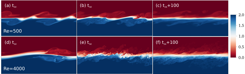
Figure 1: Contour plots of density evolution for simulation ‘ H_L ’ (top) and simulation ‘ H ’ (bottom) on the x - z plane at the spanwise midpoint of the computational domain at: t = t_{2d} ; t_{3d} , and t_{2d} + 100 , as defined in the text. While the horizontal extent of these figures illustrate L_x , which is almost twice as long in (a-c) as that in (e-f), their vertical extent is chosen to result in similar panel aspect ratio and is smaller than L_z .
