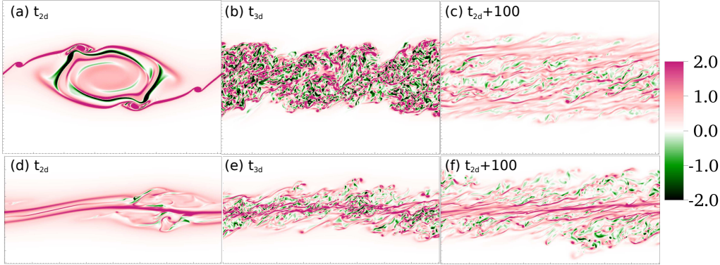
Figure 7: Contour plots of the spanwise vorticity ( \omega_y ) evolution for simulation ‘K’ (top) and simulation ‘H’ (bottom) on the x - z plane at the spanwise midpoint of the computational domain at: t = t_{2d} ; t_{3d} , and t_{2d} + 100 , as defined in the text.
