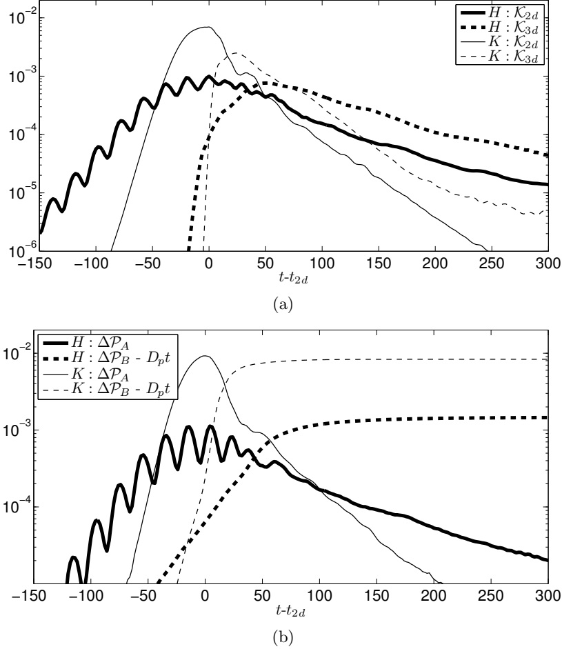
Figure 9: Time dependence for simulations ‘H’, plotted with thick lines, and ‘K’, plotted with thin lines, of: (a) the spanwise averaged kinetic energy \mathcal{K}_{2d} (solid curves) as well as the inherently three-dimensional perturbation kinetic energy \mathcal{K}_{3d} (dashed curves); (b) changes in the APE ( \mathcal{P}_A , solid) and BPE ( \mathcal{P}_B , dashed) reservoirs (2.11). For our closed system, the dashed curves also represent the cumulative amount of mixing \mathcal{M}_c(t) (2.22).
