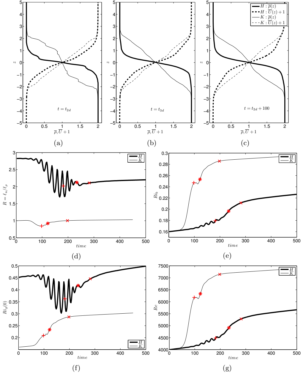
Figure 8: (a,b,c) Vertical structure of horizontally averaged density and velocity profiles (\bar{\rho}, \bar{U} + 1) for simulations 'H', plotted with thick lines, and 'K', plotted with thin lines, at times (a) t_{2d} (b) t_{3d} and (c) t_{2d} + 100 . Bottom Panels illustrate the time evolution of (d) R = \ell_u / \ell_\rho and (e) the bulk Richardson number Ri_b , (f) the gradient Richardson number at the interface, Ri_g(0) = RRi_b and (g) the Reynolds number Re based on the extended definitions in (2.29). The characteristic times t_{2d} , t_{3d} and t_{2d} + 100 are marked in (d,e,f,g) by '+', '*' and 'x' respectively.
