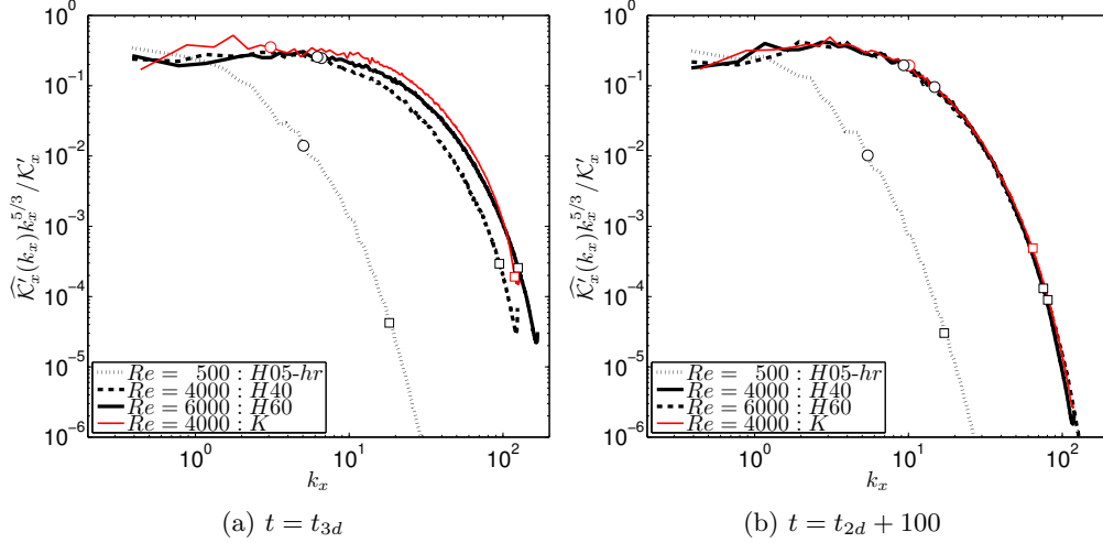
Figure 5: Compensated streamwise spectra of \widehat{\mathcal{K}}'_x(k_x, t) (2.16) after being normalized by the total streamwise perturbation kinetic energy \mathcal{K}'_x = (2\pi/L_x) \sum_{k_x} \widehat{\mathcal{K}}'_x for simulations ‘H05-hr’, ‘H40’, ‘H60’ and ‘K’. These spectra are calculated at times (a) t = t_{3d} and (b) t = t_{2d} + 100 . Similar to figure 4, \ell_O and \ell_K are marked by ‘o’ and ‘square’ respectively.
