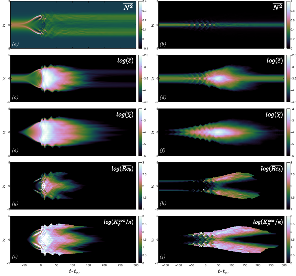
Figure 12: Time dependence of vertical profiles of horizontally averaged: (a) & (b) \overline{N^2}(z, t) ; (c) & (d) \log \overline{\varepsilon}(z, t) ; (e) & (f) \log \overline{\chi}(z, t) ; (g) & (h) \log \overline{Re}_b(z, t) ; (i) & (j) \log K_\rho^{cox}(z, t)/\kappa as defined in (3.1) for simulation ‘K’ (left column) and simulation ‘H’ (right column). For details of the colour map with monotonically increasing brightness, see Green (2011).
