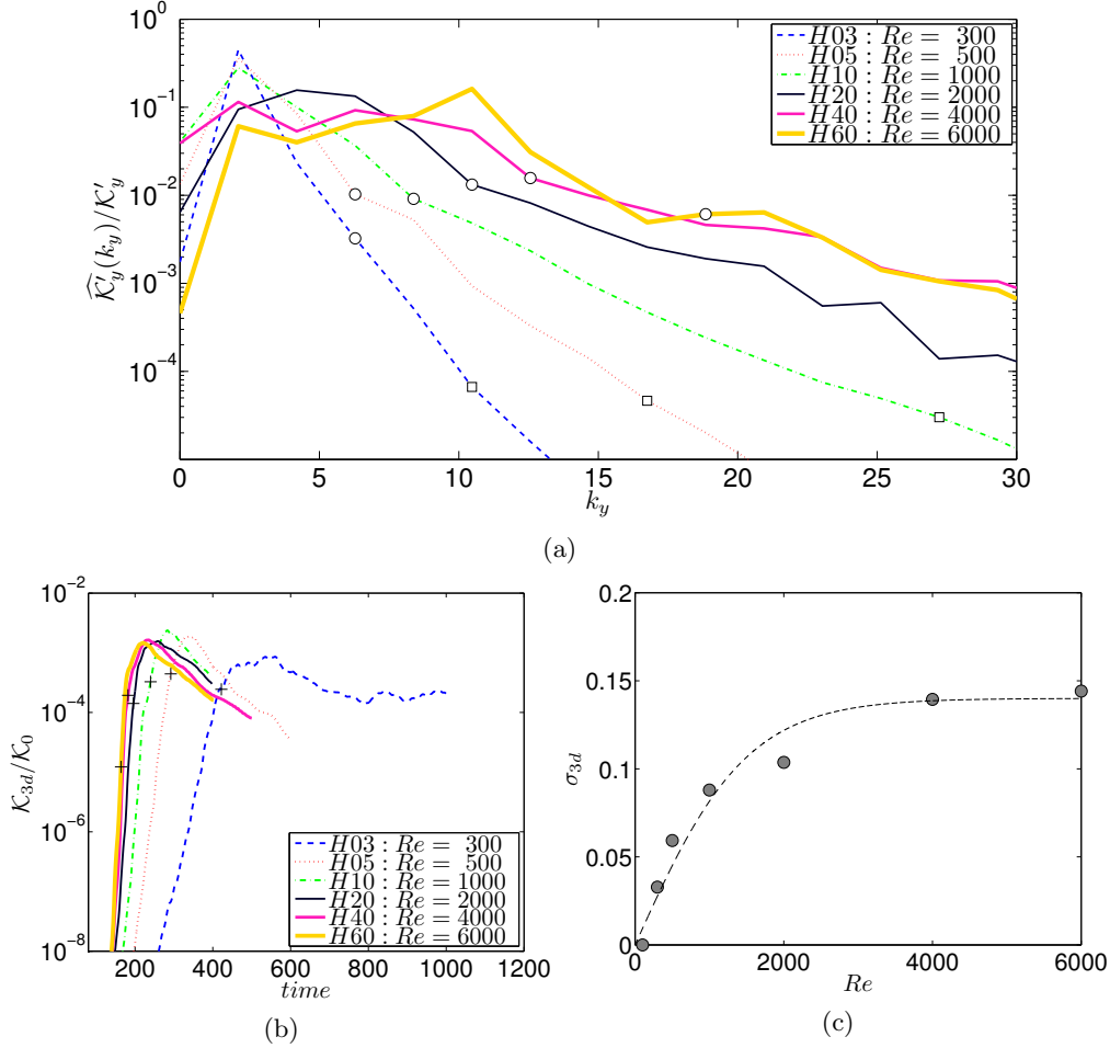
Figure 3: (a) The spanwise spectrum of spanwise kinetic energy, \widehat{\mathcal{K}}'_y(k_y) (2.17), at t = t_{2d} . ‘ \circ ’ and ‘ \square ’ (if available) mark \ell_O and \ell_K (2.31) respectively. (b) Time evolution of the three-dimensional kinetic energy, \mathcal{K}_{3d} after being normalized by the initial total kinematic energy \mathcal{K}_0 for a series of HWI simulations with different values of initial Re (see table 1). The saturation time of two-dimensional primary HWI, t_{2d} is marked by a ‘+’ for each simulation. (c) The Re -dependence of \sigma_{3d} = 1/(2\mathcal{K}_{3d})d\mathcal{K}_{3d}/dt associated with the growth rate of the three-dimensional perturbations. The dashed curve provides a sigmoid fit for illustrative purposes.
