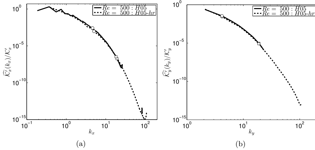
Figure 13: Comparing the effect of grid resolution on spectral representation of the perturbation kinetic energy at t = t_{3d} by employing simulations ‘H05’ and ‘H05-hr’ (both at Re = 500 , see Table 1). (a) Normalized streamwise spectra of streamwise perturbation kinetic energy, \widehat{\mathcal{K}}'_x(k_x)/\mathcal{K}'_x (see (2.16)). (b) Normalized spanwise spectra of spanwise perturbation kinetic energy, \widehat{\mathcal{K}}'_y(k_y)/\mathcal{K}'_y (see (2.17)). \ell_O and \ell_K are marked by ‘o’ and ‘□’ respectively.
