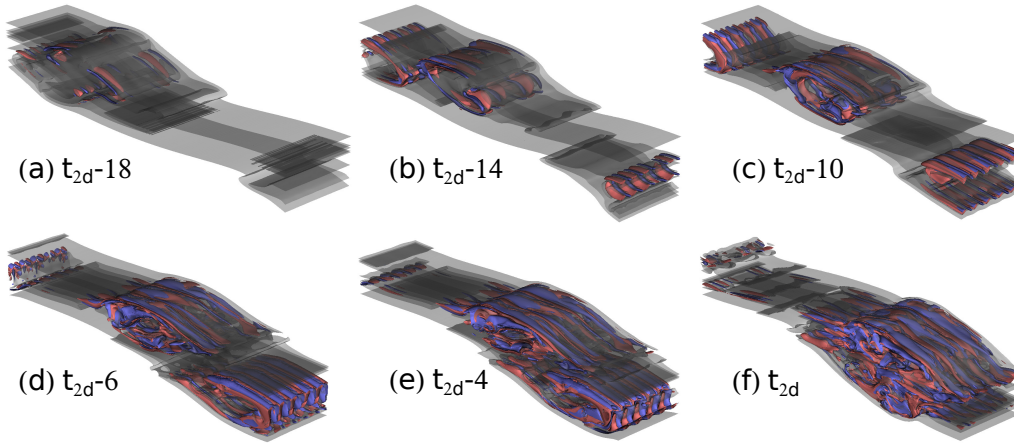
Figure 2: Three dimensional isosurfaces of streamwise vorticity, \omega_x = -0.25 (blue) and \omega_x = 0.25 (red) overlaid by an isosurface of spanwise vorticity, \omega_y = 0.5 (gray) for simulation ‘ H40 ’ at Re = 4000 during one Holmboe wave cycle starting at t_{2d} - 18 and ending at t_{2d} . The counter-propagating streamwise vortex tubes associated with the secondary shear-aligned convective instability are shown to play a significant roll during the transition to turbulence of HWI at this high Re .
