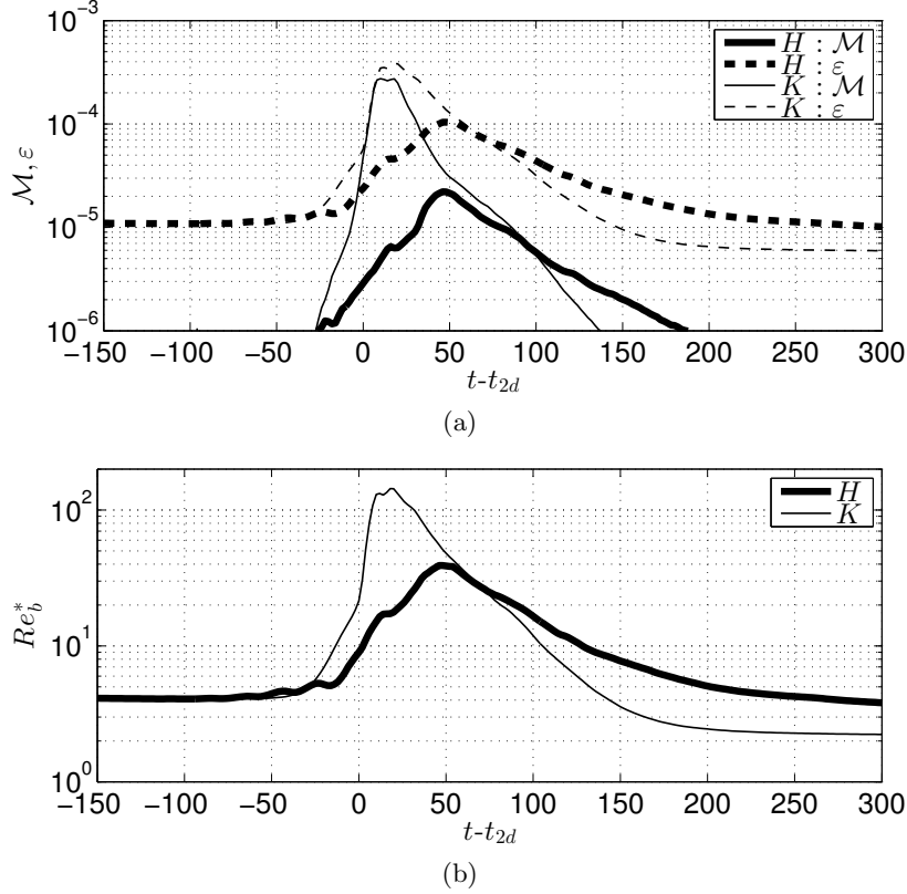
Figure 10: Time dependence for simulations ‘H’, plotted with thick lines, and ‘K’, plotted with thin lines, of: (a) irreversible mixing rate \mathcal{M} as defined in (2.18) (solid line), viscous dissipation rate and \varepsilon as defined in (2.23) (dashed line) (b) the buoyancy Reynolds number, Re_b^* as defined in (2.26).
