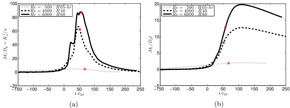
Figure 6: Time dependence for simulations ‘H05-hr’ ( Re = 500 , dotted), ‘H40’ ( Re = 4000 , dashed) and ‘H60’ ( Re = 6000 , solid) of: (a) Instantaneous mixing rate, \mathcal{M} (2.18) relative to the laminar diffusion rate D_p (2.21). (b) Cumulative irreversible mixing \mathcal{M}_c (2.22) normalized by D_p (2.21). The time t_{3d} in both (a,b) is indicated by an ‘*’.
