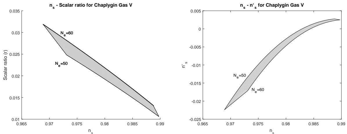
FIG. 5: The left figure is the n_s - r diagram for the model generalized Chaplygin gas V. The right figure is the n_s - n'_s diagram for the same model. The plots are for N_e \in [50, 60] , \bar{B} = -0.002 and \lambda \in [-1, 0) .
