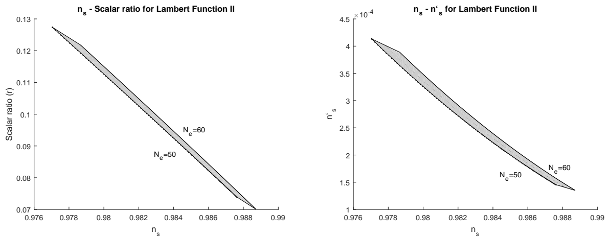
FIG. 6: The left figure is the n_s - r diagram for the model “Lambert function II”. The right figure is the n_s - n'_s diagram for the same model. The plots are for N_e \in [50, 60] and q \in [65, 100] .
