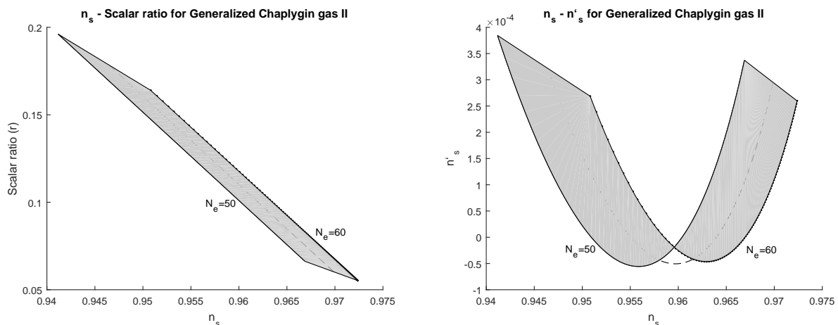
FIG. 2: The left figure is the n_s - r diagram for the generalized Chaplygin gas II model, while the right figure is the n_s - n'_s diagram for the same model. The plots are for N_e \in [50, 60] and \lambda \in [-0.5, 0.5] .
