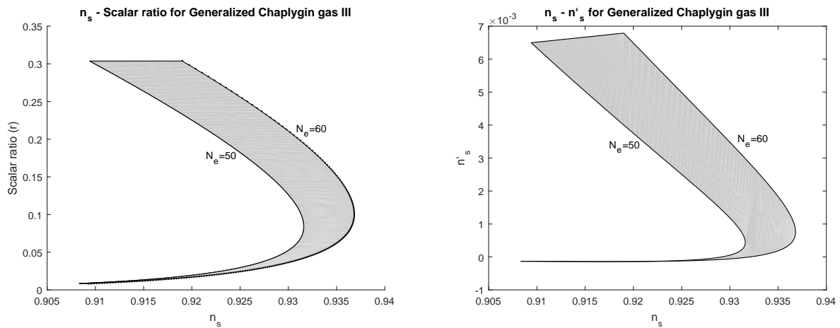
FIG. 3: Left figure is the n_s - r diagram for the generalized Chaplygin gas III model, while the right figure is the n_s - n'_s diagram for the same model. The plots are for N_e \in [50, 60] and \lambda \in [-1.03, -1.01] , with F_1 = -1.0001 .
