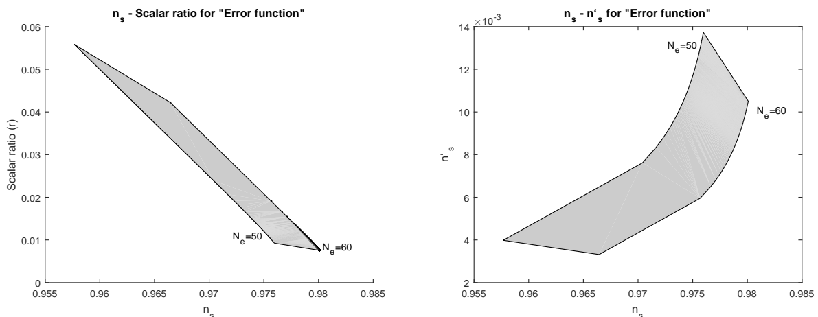
FIG. 7: The left figure is the n_s - r diagram for the model “Error Function”. The right figure is the n_s - n'_s diagram for the same model. The plots are for N_e \in [50, 60] and AB \in [-100, -0.02] .
