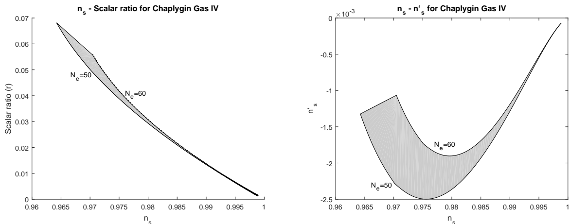
FIG. 4: Diagrams r = r(n_s) (left figure) and n'_s = n'_s(n_s) (right figure) for the generalized Chaplygin gas IV model for number of e-folds in the range N_e \in [50, 60] , for A = 1 and free parameter B in the range B \in [-10, 100] .
