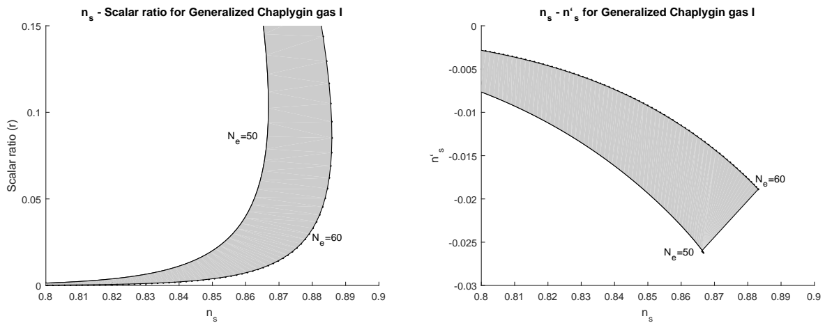
FIG. 1: Diagrams r = r(n_s) (left figure) and n'_s = n'_s(n_s) (right figure) for the generalized Chaplygin gas I model for number of e-folds in the range N_e \in [50, 60] .
