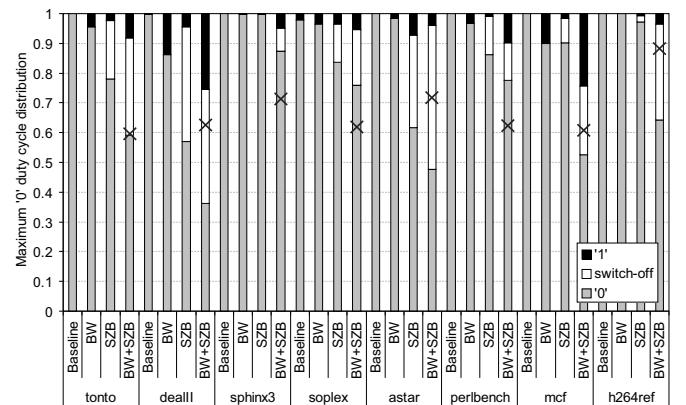
Fig. 11. Maximum '0' duty cycle distribution on the entire cache across all the studied applications. The cross symbol refers to the longest '0' duty cycle in the control bits.
