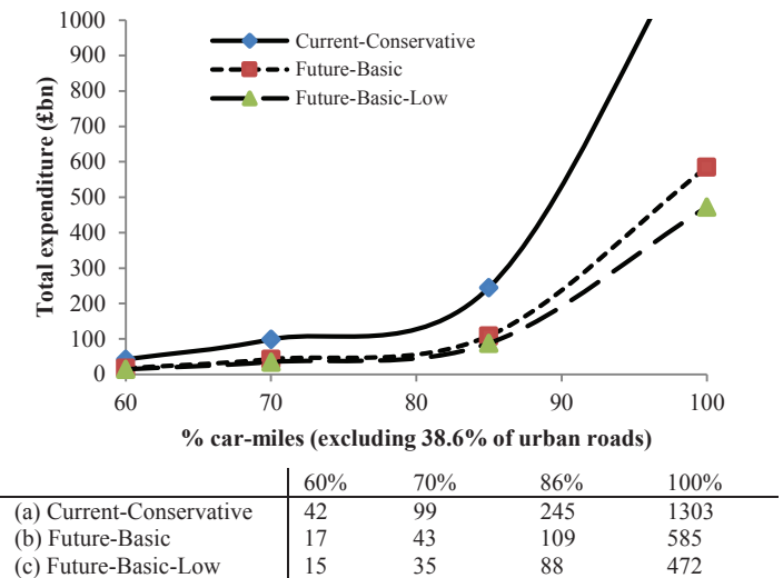
Fig. 2. Total expenditure (£bn) to install IPT devices relative to the percentage of electrified car-miles covered in the UK
