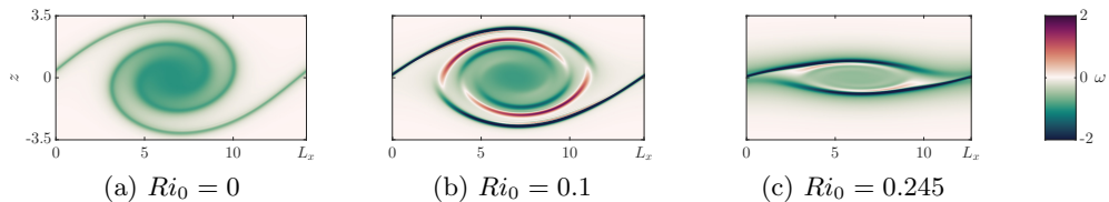
FIGURE 2. Snapshots of spanwise vorticity \omega = \partial_x w - \partial_z u at times t = t_{\max} for class S simulations with: (a) Ri_0 = 0 ; (b) Ri_0 = 0.1 ; and (c) Ri_0 = 0.245 .
