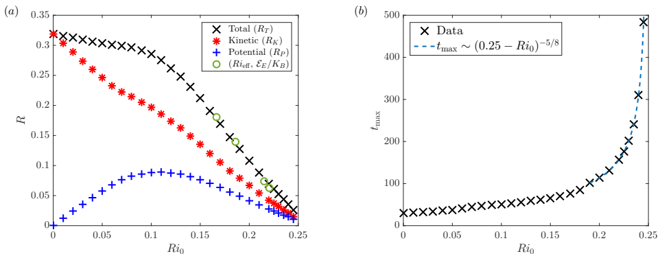
FIGURE 3. For class S simulations, variation with Ri_0 of: (a) scaled maxima of total perturbation energy R_T (crosses), perturbation kinetic energy R_K (asterisks) and perturbation potential energy R_P (pluses) as defined in (3.2); (b) t_{\text{max}} . In (a) circles mark Ri_{\text{eff}} and the maximum value of \mathcal{E}_E/K_B for class A simulations as discussed in section 3.3.
