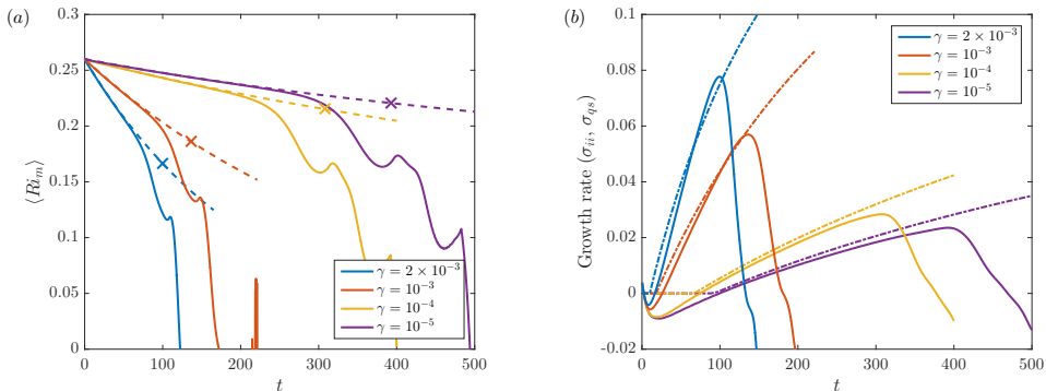
FIGURE 4. (a) Time series of minimum measured Richardson number \langle Ri_m \rangle from unperturbed (dashed lines) and growing (solid lines) simulations in the accelerating regime. The crosses indicate the value of Ri_{eff} for each simulation, at the time t_p . (b) Time series of predicted growth rate \sigma_{qs} from quasi-steady linear analysis (dash-dot lines) and inferred instantaneous growth rate \sigma_{ii} as defined in (3.6) (solid lines) for various forcing rates \gamma . The time t_p is defined as the instant when \sigma_{ii} is maximum.
