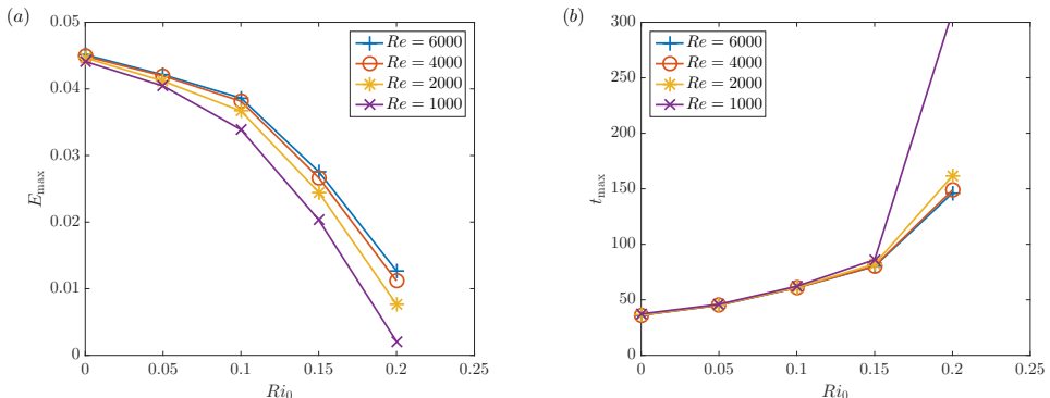
FIGURE 1. For class D simulations, variation with Re and Ri_0 of (a) peak energy E_{\max} and (b) time to saturation t_{\max} .
