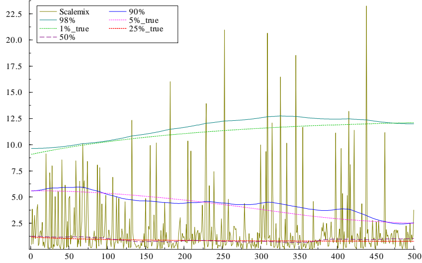
Figure 7: Absolute values of simulated series, true quantiles and random walk 98%, 90% and 50% quantiles fitted by CV.
