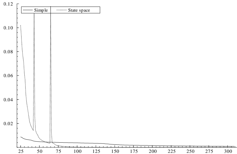
Figure 2: Behaviour of the convergence criterion C^{(j)} \times 10^4 , iterations 25 through 300.
