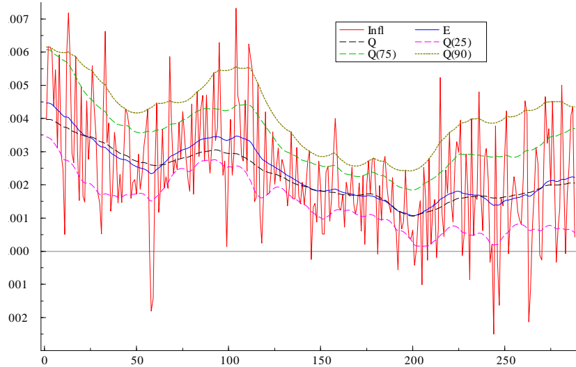
Figure 4: Time-varying quantiles and mean fitted to monthly US inflation
