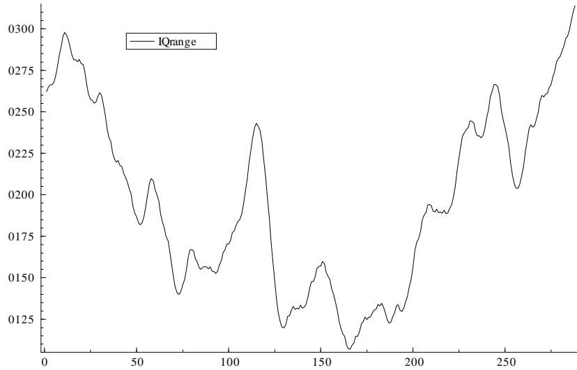
Figure 5: Interquartile range for monthly US inflation from 1981(7) to 2005(6).
