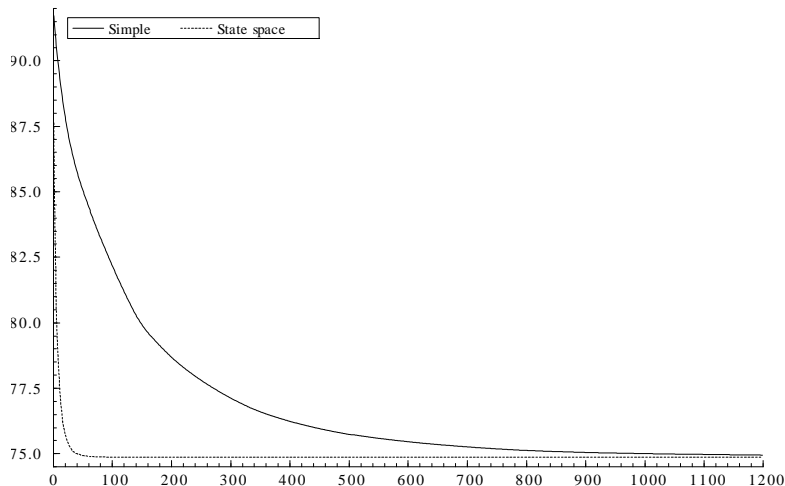
Figure 3: Objective function J (iterations 1 to 1200).
