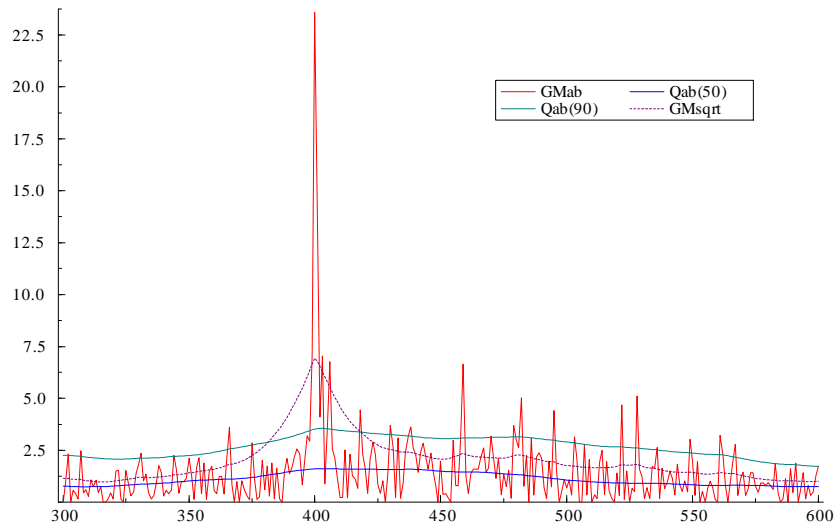
Figure 6: 25% and 5% quantiles estimated from absolute values of GM returns, together with SD from smoothed squared observations
