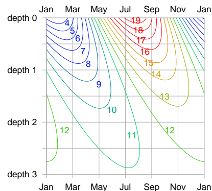
Figure E.17. Temperature (in ^{\circ}\text{C} ) versus depth and time. The depths are given in units of the characteristic depth z_0 , which for granite and annual variations is 3 m.
