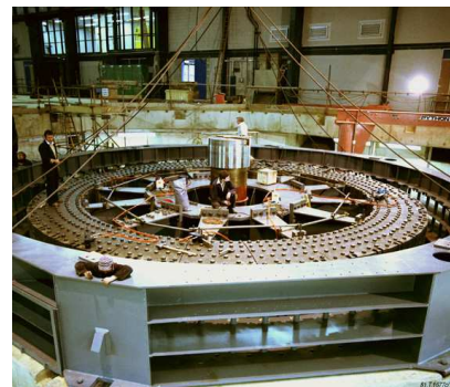
Figure 26.15. One of the two flywheels at the fusion research facility in Culham, under construction. Photo: EFDA-JET. www.jet.efda.org .
