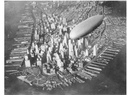
Figure C.14. The 239 m-long USS Akron (ZRS-4) flying over Manhattan. It weighed 100 t and could carry 83 t. Its engines had a total power of 3.4 MW, and it could transport 89 personnel and a stack of weapons at 93 km/h. It was also used as an aircraft carrier.
