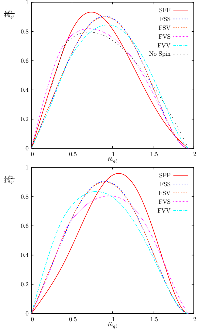
Fig. 2. Invariant mass distributions for SPS 1a: Process 1 (top) and Process 2 (bottom).
