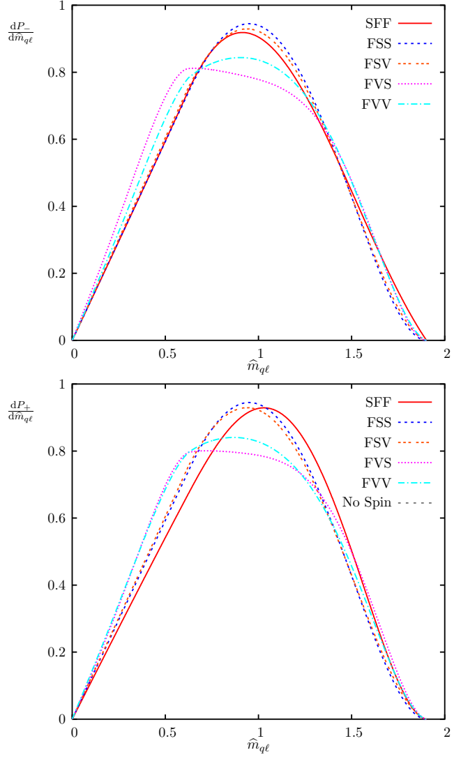
Fig. 6. Observable invariant mass distributions for SPS 2: P_- (top) and P_+ (bottom), see equation (3).
