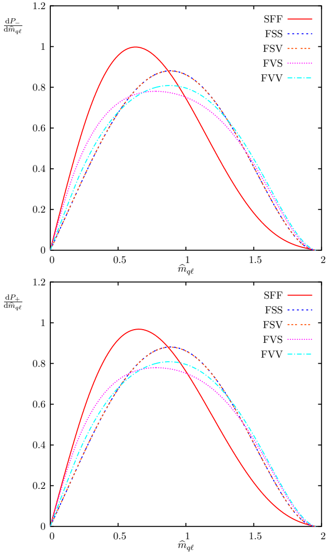
Fig. 7. Observable invariant mass distributions for SPS 9: P_- (top) and P_+ (bottom), see equation (3).
