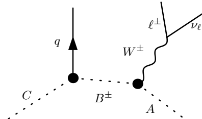
Fig. 1. The decay chain under consideration.
