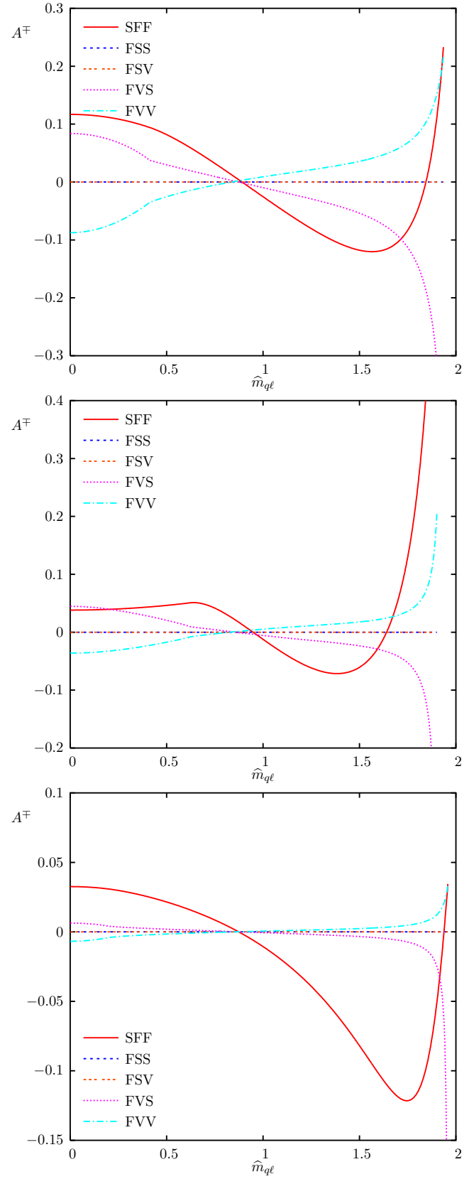
Fig. 8. Asymmetry plots for SPS 1a (top), SPS 2 (middle) and SPS 9 (bottom).
