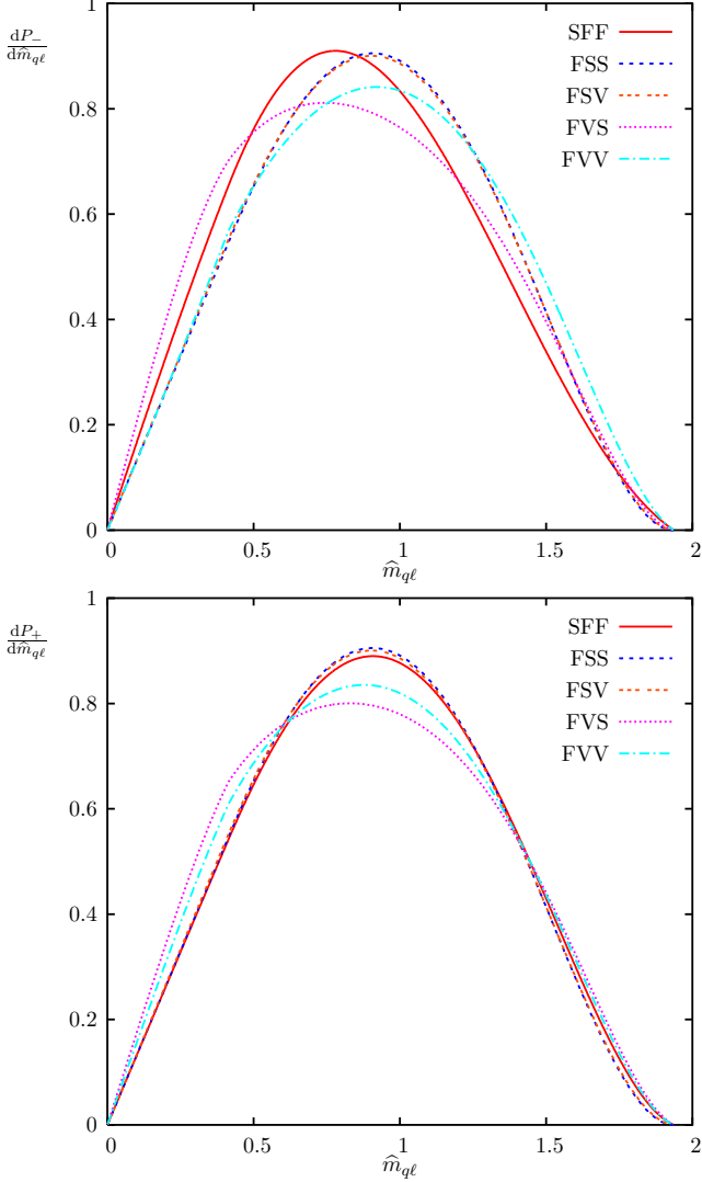
Fig. 5. Observable invariant mass distributions for SPS 1a: P_- (top) and P_+ (bottom), see equation (3).
