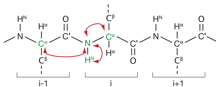
(c) HNCA
