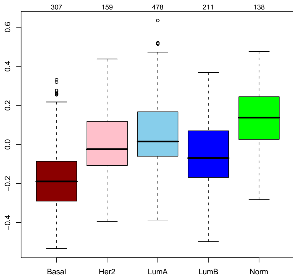
ERBB2 -pearson
