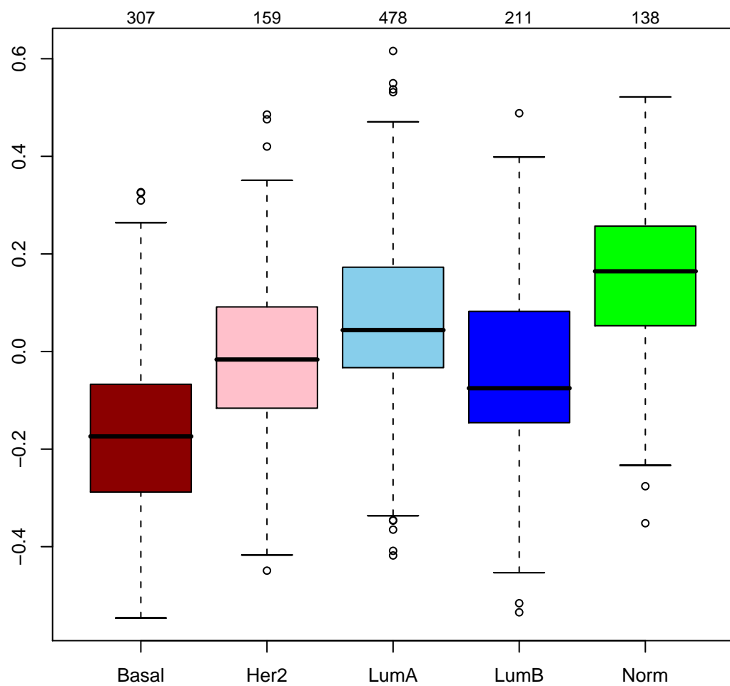
ERBB2 -spearman
