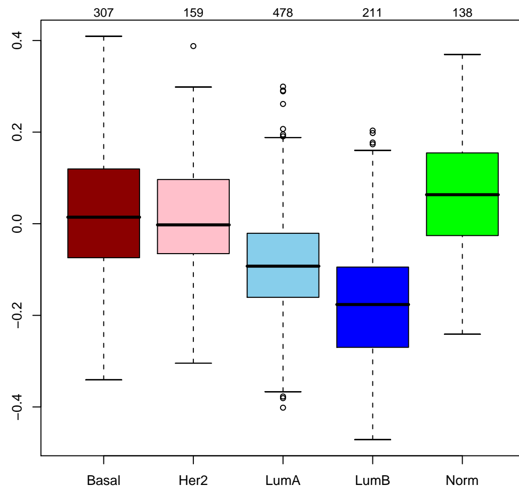
EGFR -spearman
