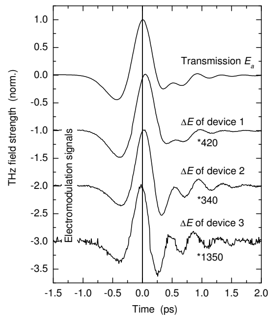
FIG. 2. Time-resolved field E_a(t) after transmission through device 1 and modulation signals \Delta E(t) for devices 1, 2, and 3. Transient transmission signals for devices 2 and 3 are not shown, because they are similar to E_a(t) recorded on device 1. The modulation signals are offset for clarity. All modulation signals are recorded by depleting the devices. Experiments performed by accumulating electrons in the GaN yield nearly identical results.
