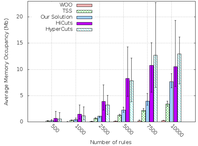
Fig. 4. Comparison of Memory Occupancy between chosen algorithms for different datasets
