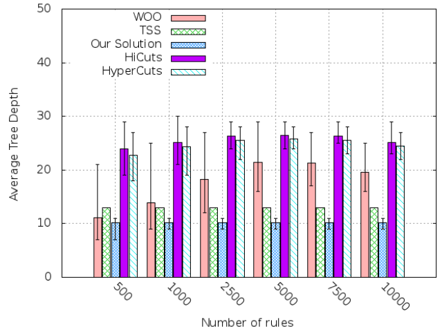
Fig. 5. Comparison of Tree Depth between chosen algorithms for different datasets
