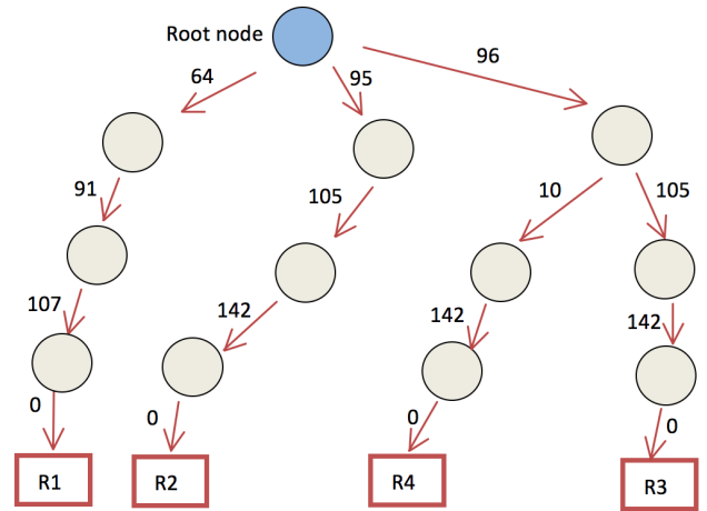
Fig. 2. Example of standard JA-Trie
