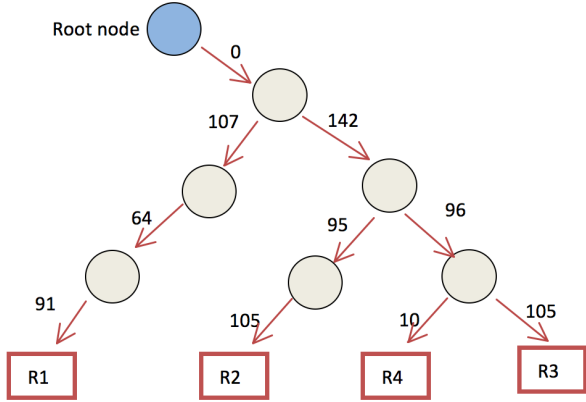
Fig. 3. Example of Entropy-Based-JA-Trie
