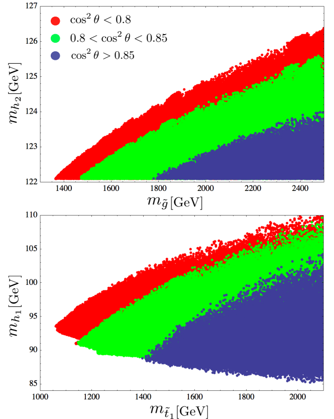
FIG. 1: (Upper panel) SM-like Higgs mass vs. gluino mass and (Lower panel) singlet-like Higgs mass vs. lightest stop mass. The various model points are distinguished by the Higgs-singlet mixing angle \theta , which decreases from top to bottom as specified in the upper panel. For the same SM-like Higgs mass a larger mixing angle allows for much lighter gluinos. The lightest stop masses are obtained for a singlet-like Higgs around 94 GeV.
