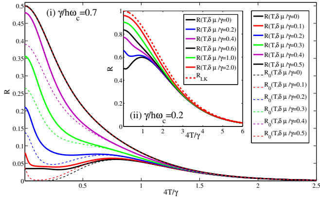
Figure 2: (color online.) Temperature dependence of the damping factor R(T) . In (i) it is shown for \frac{\gamma}{\hbar\omega_c} = 0.7 and for different values of the chemical potential, \mu = W = \delta\mu , parametrized by \frac{\delta\mu}{\gamma} . Dashed lines are calculated from the approximate R_0(T) in which \Gamma is replaced by \Gamma_0 = \Gamma(n=0) . The inset (ii) shows the same for a different value \frac{\gamma}{\hbar\omega_c} = 0.2 . In this case R_0(T) always coincides with the exact R(T) . Note that for large values of \frac{\delta\mu}{\gamma} the standard Lifshitz-Kosevich behaviour R_{LK} (red dashed) is quickly approached.
