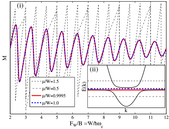
Figure 1: (color online.) Main figure (i), Quantum oscillations of the magnetization, M , as a function of W/h\omega_c \propto 1/B . Inset (ii), sketch of the band structure for our model (exaggerated hybridization gap for better visibility) and positions of the different chemical potentials \mu . If \mu , is far away from the gap (black dashed and dot dashed), which is opened by hybridizing a localized flat band with an itinerant band, the periodicity of standard QO is proportional to the extremal cross section of the Fermi surface (here directly related to \mu = \frac{S}{2\pi m} with the area S = \pi k_F^2 ). We find that even if \mu is inside the gap (blue dashed) or in the flat band region (red) there are well defined QO which are directly proportional to the area picked out by the intersection of the unhybridized bands (here directly proportional to W/h\omega_c ).
