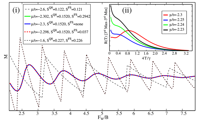
Figure 3: (color online.) QO oscillations for a tight-binding lattice model with W = -2.3 and \gamma = 0.2 (all energies in units of t ). The periodicity F_{\mu} of the oscillations corresponds to a relative FS area S^{QO} (which is here measured in units of the BZ size 4\pi^2 ). In the main figure (i) for T=0 it is confirmed that as long as the chemical potential is far away from the gap (black dashed and dot dashed) the FS area, S^{QO} extracted from the QO period nicely reproduce the area S^{FS} obtained from the relative BZ area of the FS for zero field, see legend. If \mu is inside or close to the gap (green, blue, red dashed) we find anomalous QO as before with a periodicity not related to S^{FS} . In the inset (ii), we extracted the temperature dependence R(T) by calculating the difference between a consecutive minimum and maximum of M as a function of temperature, which confirms the analytical behaviour of Eq. (2), compare to Fig. 2.
