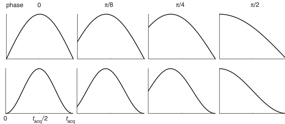
Fig. 4.13 The top row shows sine bell and the bottom row shows sine bell squared weighting functions for different choices of the phase parameter; see text for details.
