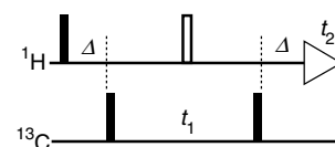
The pulse sequence for HMQC. Filled rectangles represent 90^\circ pulses and open rectangles represent 180^\circ pulses. The delay \Delta is set to 1/(2J_{12}) .
