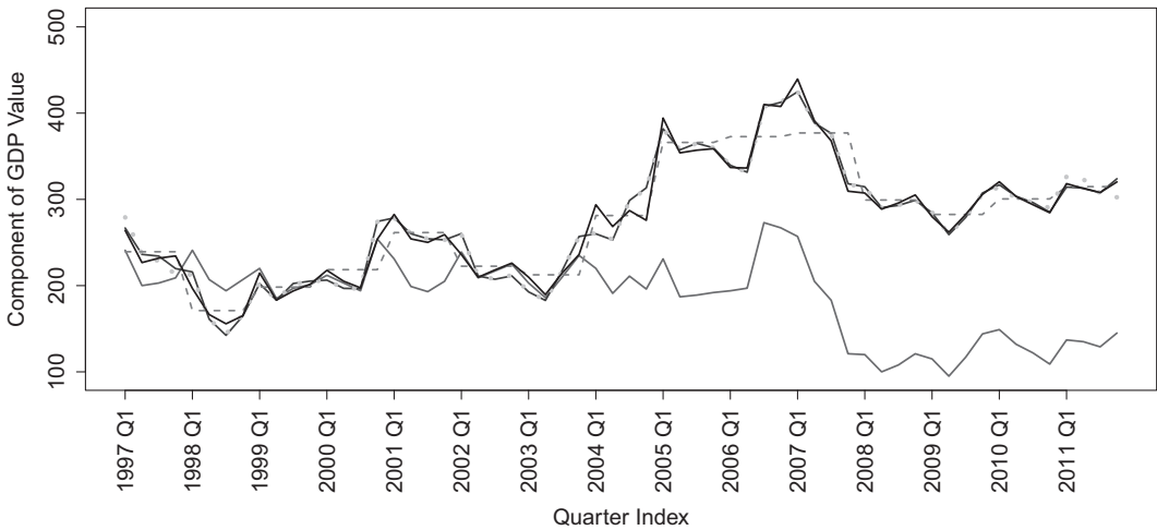
Fig. 5. Application of various benchmarking methods to components of the UK GDP data: —, quarterly component of GDP series; —, wavelet benchmarked series; —, Denton benchmarked series; ····, Cholette and Dagum benchmarked series; - · - ·, quarterly form of annual component of GDP series
