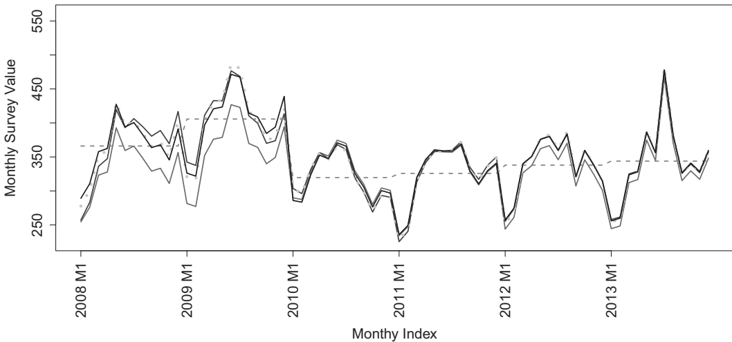
Fig. 6. Application of various benchmarking methods to business survey data on the turnover of companies manufacturing soft drinks and bottled water: —, monthly component; — — —, wavelet benchmarked series; ·····, Denton benchmarked series; · · · · ·, Cholette and Dagum benchmarked series; - - - -, monthly form of annual component
