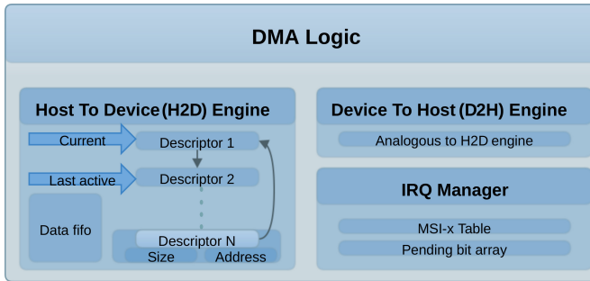
Fig. 4: Hardware level implementation of DMA logic
