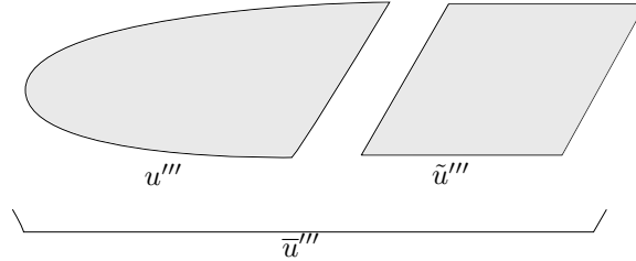
FIGURE 3. The discs u''' \subset M , \tilde{u}''' \subset \partial^0 M \times [0, 1] and \bar{u}''' \subset M_1 := M \cup \partial^0 M \times [0, 1] . The subsets u' , \tilde{u}' and \bar{u}' are tubular neighbourhoods of them.
