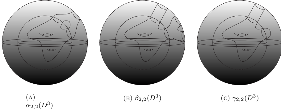
FIGURE 1. The three basic types of stabilisation maps acting on a surface in the space \mathcal{E}(\Sigma_{2,2}, D^3; \delta) of surfaces in the disc of dimension 3.
