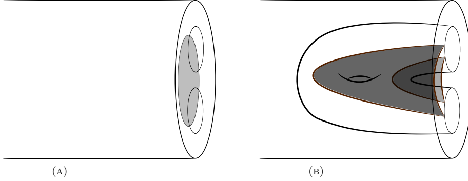
FIGURE 2. (a) A background manifold M = D^2 \times [0, 1] , a boundary condition consisting of two circles, and an embedded ball \ell (in grey) that intersects the circles in two intervals. (b) A 1-simplex in the boundary resolution.
