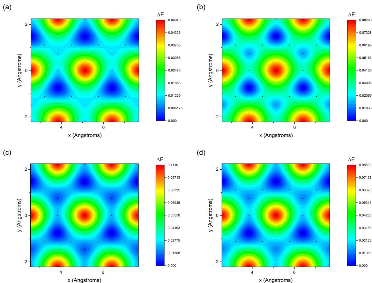
Figure 3 Potential energy surfaces derived from the DFT calculations with (a) G06 24 , (b) OBS 25 , (c) TS 26 and (d) TSSCS 33 vdW corrections.
