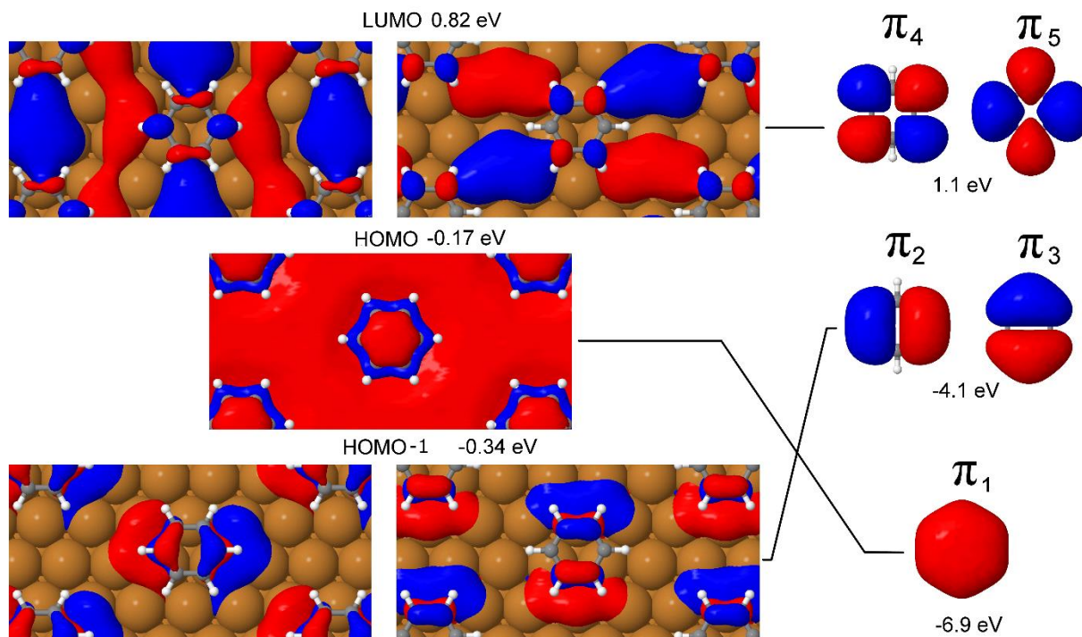
Figure 5 Left, LUMO (0.82 eV), HOMO (-0.17 eV) and HOMO-1 (-0.34 eV) Kohn-Sham orbitals (KS-MOs) at the gamma point for benzene adsorbed on a hollow hcp site. Right, from top to bottom, symmetry related pi orbitals for isolated benzene. The KS-MOs of the surface are joined by the solid lines with the symmetry equivalent pi orbitals of benzene. The \pi_3 , \pi_2 and \pi_1 orbitals are much lower in energy than the correspondent surface mixed-character KS-MOs and the represented beside the latter for purpose of easy visualisation.
