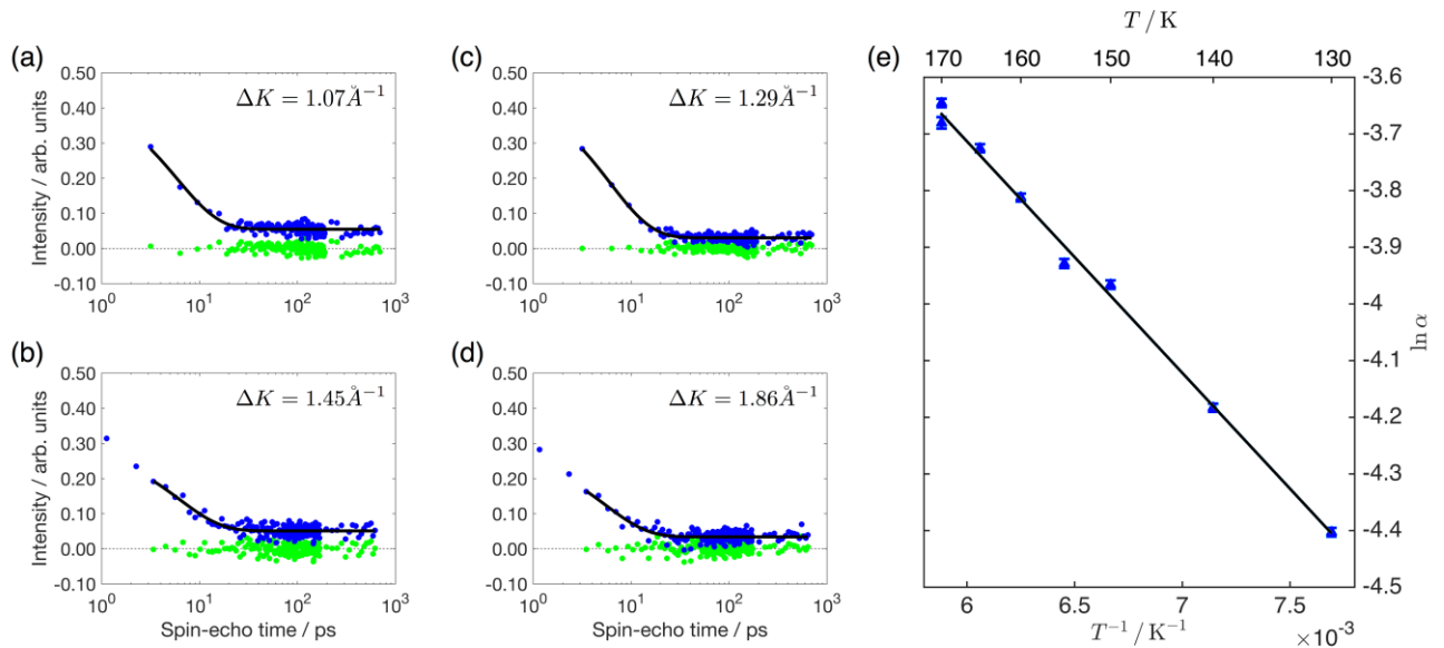
Figure 2 Polarisation measurements as a function of spin-echo time, t , for 0.03 ML (panels a,c) and 0.1 ML (panels b,d) of benzene/Cu(111). The different panels show measurements at the indicated momentum transfers and a temperature of 170 K. Experimental data are plotted as blue points, a single exponential of the form f(t) = a \cdot \exp(-\alpha t) + c from 3 ps is shown as a black line and the residual after subtracting the exponential from the data as green points. Data at times smaller than 3 ps is excluded as it is influenced by the initial fast decay described in the text. Panel (e) shows the temperature dependence of the dephasing rate for a coverage of 0.03 ML at \Delta K = 0.3 \text{ \AA}^{-1} as an Arrhenius plot. The solid line illustrates the fit to an Arrhenius form, resulting in an effective activation energy of 35 \pm 1 meV. All data were measured along the [1\bar{1}\bar{2}] direction.
