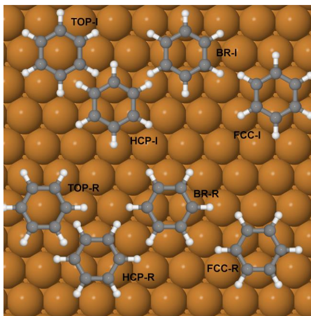
Figure 1 Schematic representation of benzene adsorbed on high symmetry adsorption sites in the two angular orientations (0 and 30 degrees with respect to the \langle 1\bar{1}0 \rangle direction) considered in this work. In our notation, I = 0 degrees rotation and R = 30 degrees rotation.
