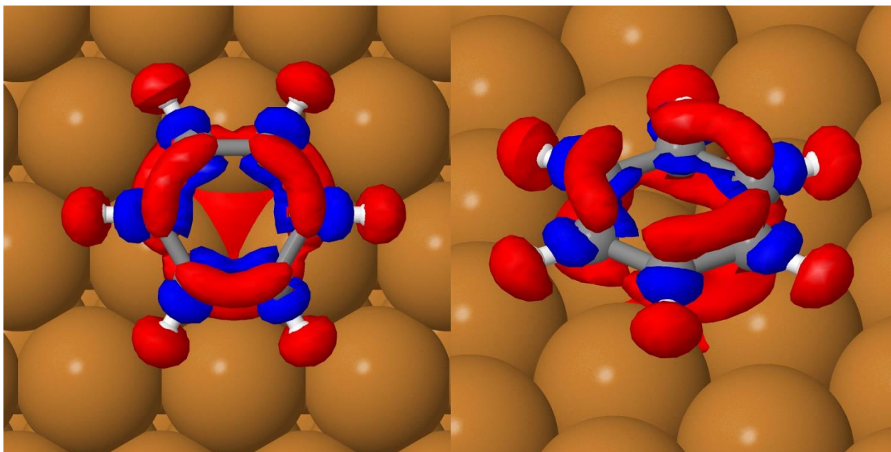
Figure 4 Top view (left) and side view (right) of charge density difference plots showing charge transfer upon adsorption of benzene on the Cu(111) hcp site in the HCP-R rotational configuration. Red contours indicate electron density increase by 0.005 electrons/Å 3 ; blue contours indicate electron density decrease by 0.005 electrons/Å 3 .
