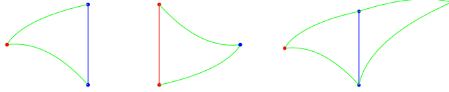
Figure 3: Refined or green edges split the map and its dual into primal and dual triangles. Each primal triangle sits opposite another primal triangle, resulting in a primal quadrangle as above.
