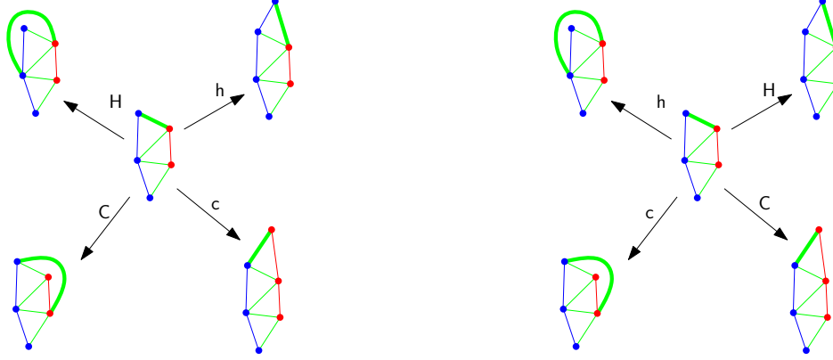
Figure 4: From symbols to map. The current position of the interface (or last discovered refined edge) is indicated with a bold line. Left: reading the word sequence from left to right or into the future . The map in the centre is formed from the symbol sequence chc . Right: The corresponding operation when we discover the sequence from right to left (or into the past ). The map in the centre now corresponds to the symbol sequence CHC .
