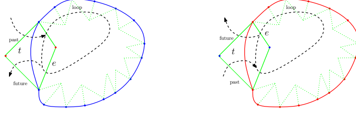
Figure 5: The envelope of an F symbol matched to a c. The green quadrangle corresponds to the F and its match. All the other blue edges on the boundary of the envelope correspond to the symbols H in the reduced word \mathcal{R} . Note that not all triangles on the boundary of the envelope are part of the loop itself. Right: the corresponding map if the F symbol is matched with an h.
