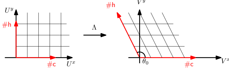
Figure 6: The coordinate transformation. Note that in the new coordinates, leaving the cone \mathcal{C}(\theta_0) (in red in the picture) at some time n corresponds to having eaten all burgers of a given type between times 0 and n .
