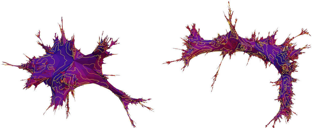
Figure 1: FK-weighted random map and loops for q = 0.5 (left) and q = 2 (corresponding to the Ising model, right). The shade of loops indicates their length (dark for short and light for long loops).
