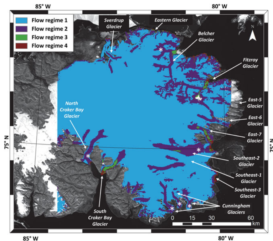
Fig. 4. Flow regime map of Devon Ice Cap overlain on a Landsat-7 image mosaic acquired 29 July and 2 August 2000. ‘*’ indicates areas classified as flow regimes different from those derived by Burgess and others (2005) (FR1, indicates ice frozen to its bed, motion by internal deformation only; FR2, indicates basal ice approaching pressure-melting point, enhanced motion; FR3, indicates reduction in ice viscosity, greater basal contribution to ice motion; FR4, high basal motion, deformation of basal sediments).
