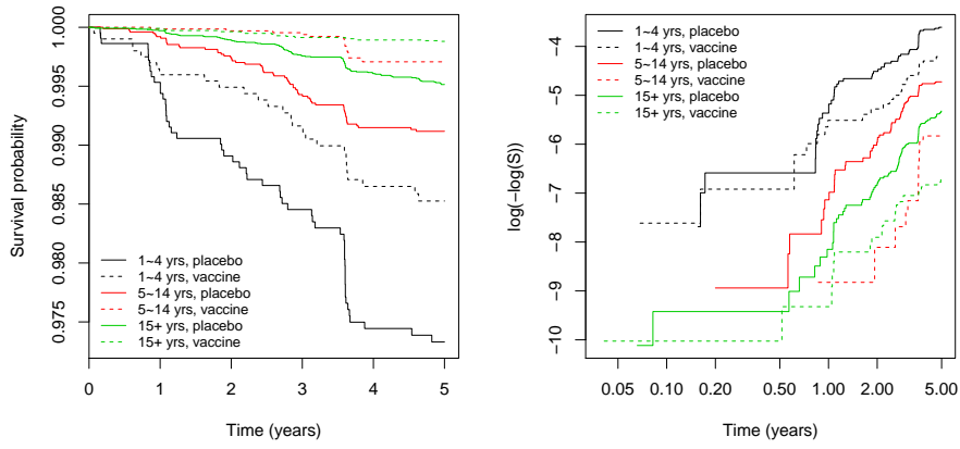
Figure S1 Survival curves stratified by age group at baseline, full dataset.
