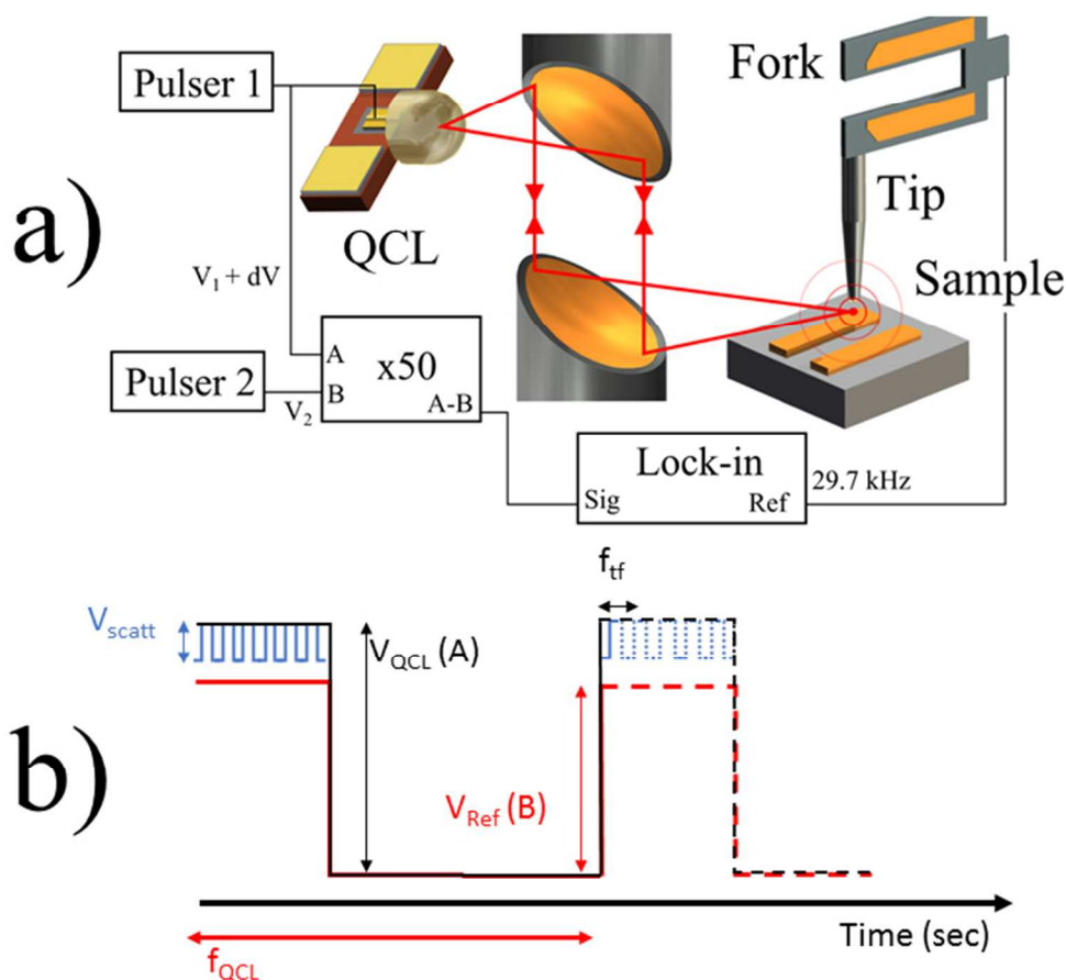
Figure 1. a) Schematic of the apparatus setup. The tuning fork oscillation frequency was set as the reference frequency of the lock-in amplifier. The tip/tuning fork system is arranged in order to operate in tapping mode. The input of the lock-in amplifier was given by the amplified voltage difference between the bias applied to the QCL and another, frequency synchronized, pulser. b) Acquisition scheme with the self-mixing technique. The scattered light into the cavity yields a reduction in the bias applied to the QCL V_{\text{QCL}} oscillating at the reference frequency of the tuning fork V_{\text{tf}} . This is compared to the bias of a second pulser V_{\text{Ref}} before being amplified.
