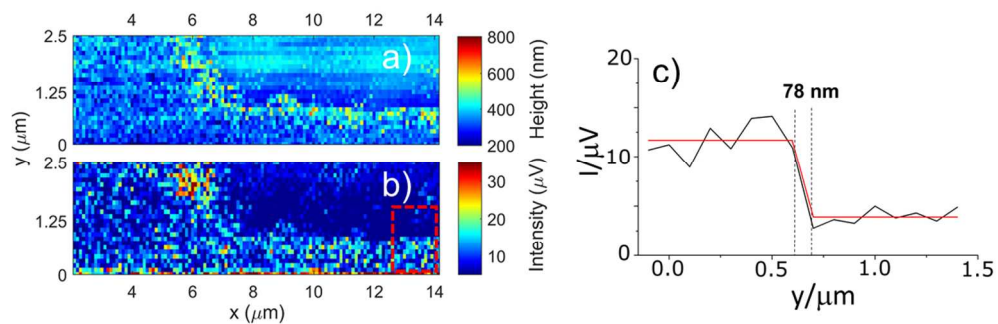
Figure 3. Topography a) and THz image b) acquired with 100 nm step-size of the metallic features shown in Fig. 2. From the profiles extracted in the dashed area in b) it was possible to obtain an estimation of the spatial resolution of the system c), calculated to be 78 nm, corresponding to > \lambda/1000 .
