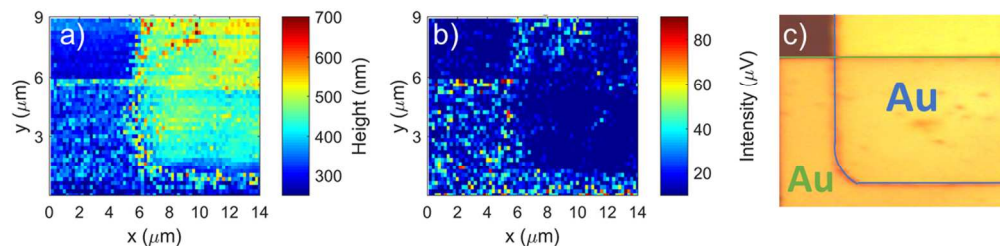
Figure 2. Topography a) and THz image b) of metallic features on SiO 2 substrate acquired with a step size of 200 nm. c) Optical micrograph of the region of interest showing the overlap between two metallic evaporations, over a SiO 2 substrate (top left corner). The metallic region defined with optical lithography (Ti/Au 10/500 nm) is reported in blue. The metallic area fabricated with electron beam lithography (Ti/Au, 80/20 nm) is indicated in green
