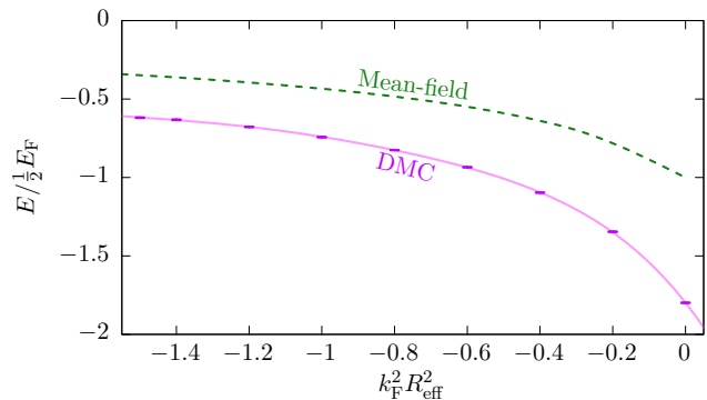
FIG. 7. (Color online) DMC ground-state energy per particle in units of that of a noninteracting gas as a function of the dimensionless effective range squared k_F^2 R_{\text{eff}}^2 shown by the solid purple line. The mean-field result is shown by the dashed green line.
