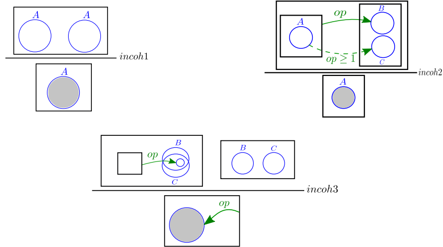
Figure 4: Incoherence examples.
