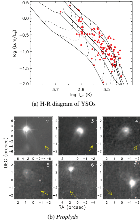
Fig. 1: (a) H-R diagram of YSOs in NGC 1977 (Fang et al. in prep.). The isochrones and evolutionary tracks are from Baraffe et al. (2015). Isochrones shown in the panel are 0.5, 1, 3, 6, 50 Myr and the evolutionary tracks are 0.04, 0.08, 0.1, 0.2, 0.4, 0.6, 0.8, 1.0, 1.4 M_{\odot} . (b) Six of the 7 proplyds in NGC 1977 (Kim et al. 2016). Yellow arrows indicate the direction toward 42 Ori. Proplyds 4 and 5 show resolved disks of sizes 50-70 au, and the central objects are likely very low mass sub-stellar objects.
