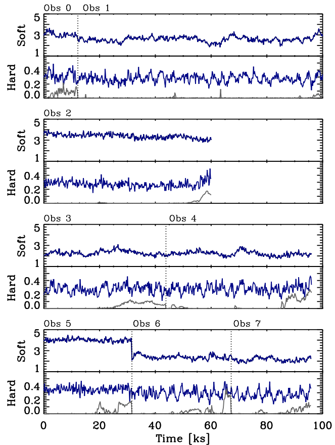
Figure 1. Soft (0.3–0.8 keV) and hard (1.0–4.0 keV) background-subtracted source (blue) and background (grey) light curves (pre-clipped) for all the XMM-Newton observations listed in Table 1.
