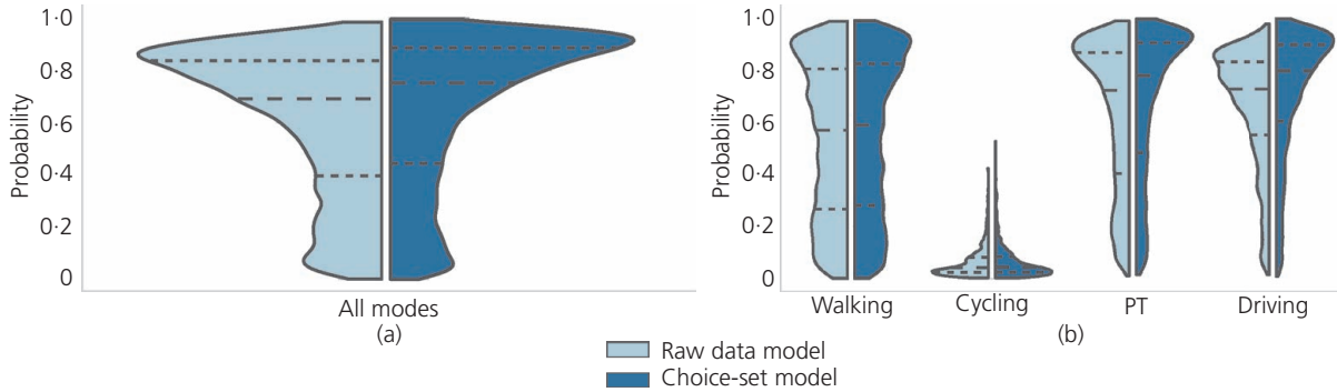
Figure 5. Violin frequency plots of predicted mode choice probabilities for raw data and choice-set modes for (a) all modes combined (predicted probability of chosen mode) and (b) separated by transport mode (predicted probability of chosen mode). Dashed lines mark median and interquartile ranges of each distribution. PT, public transport
