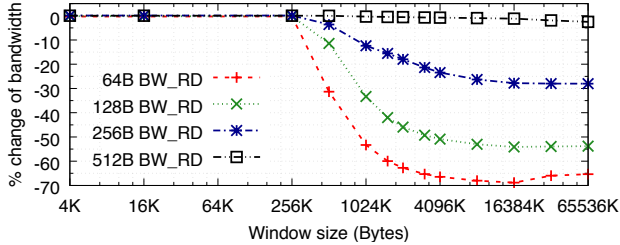
Figure 9: Impact of IOMMUs on DMA reads of different transfer sizes with warm caches (NFP6000-BDW).
