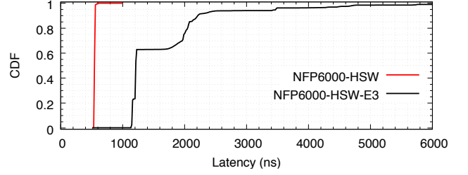
Figure 6: Latency distribution for Xeon E5 and E3 for 64B DMA reads with warm caches.
